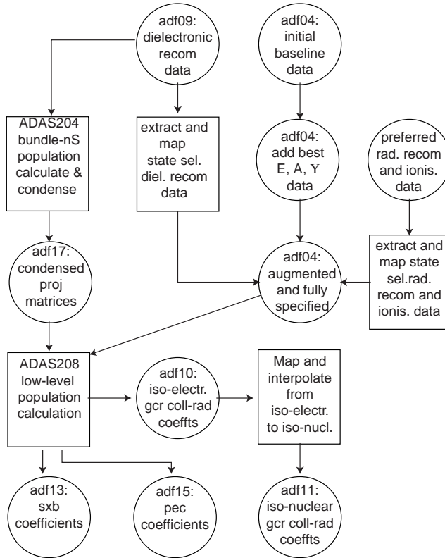
Figure 11. Schematic of computational steps in production of generalised collisional-radiative data. Data sets are shown by circular outline and program elements by rectangles. The key members have been incorporated and assigned names in the ADAS system.
