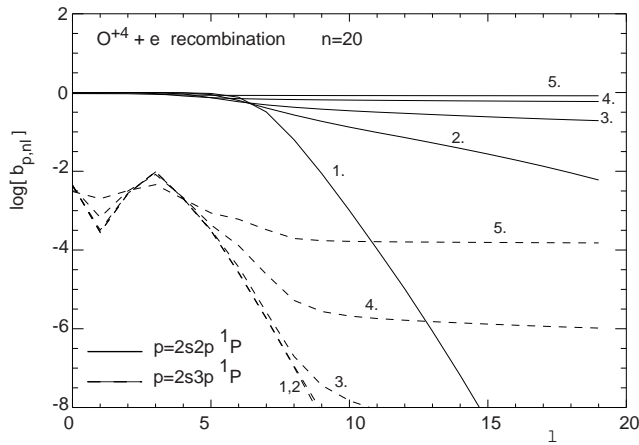
Figure 6. O^{4+} dielectronic recombination. b_{p,nl} factors as a function of outer electron orbital angular momentum l for doubly-excited states of O^{3+} relative to O^{4+} 2s^2 1S for p = 2s2p 1P and 2s3p 1P , n = 20 , T_e = 10^6 K, N_e = N_p , Z_{eff} = 1 . Cases: 1. N_e = 10^{10} \text{ cm}^{-3} ; 2. N_e = 10^{12} \text{ cm}^{-3} ; 3. N_e = 10^{13} \text{ cm}^{-3} ; 4. N_e = 10^{14} \text{ cm}^{-3} ; 5. N_e = 10^{15} \text{ cm}^{-3} . Note the alternative Auger channel reduction for the p = 2s3p 1P graphs.
