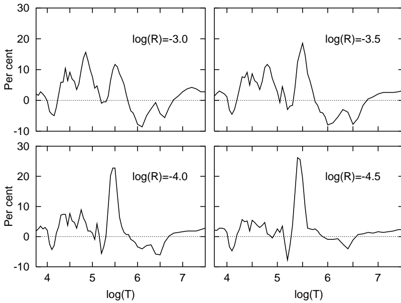
Figure 4. As Figure 3, for \log(R) = -3 to -4.5 .
