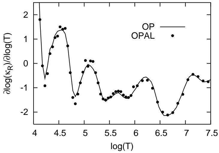
Figure 5. Values of \partial \log(\kappa_R) / \partial \log(T) (at constant R ) approximated using first derivatives. From OP and OPAL for \log(R) = -2 .
