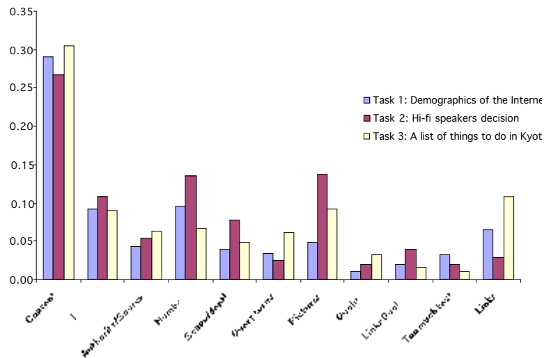
Figure 2. Feature mentions across tasks
