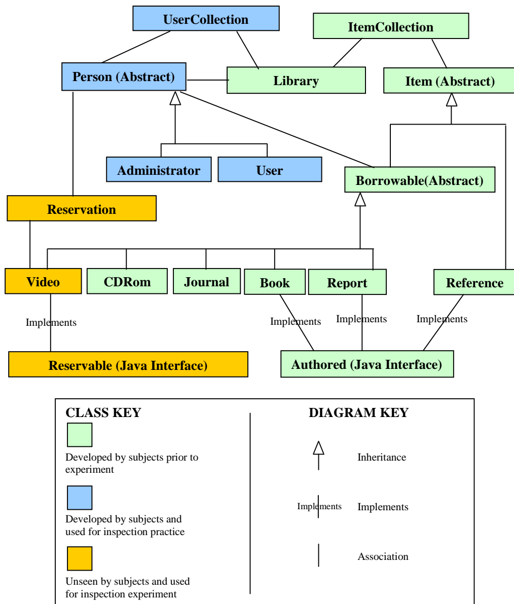
Figure 3.1 – Class hierarchy diagram for library system
