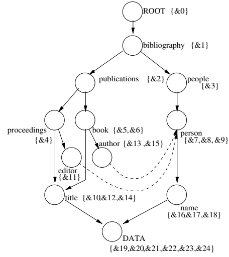
Fig. 2. (2,0)-F+B-index graph of Figure 1
