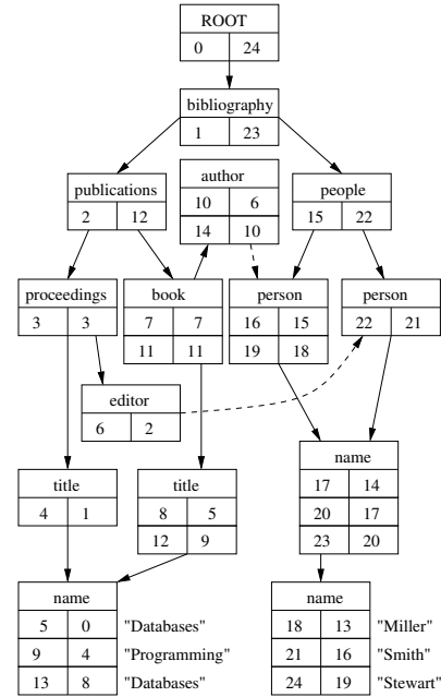
Fig. 4. NSGraph – combining structural and signature information
