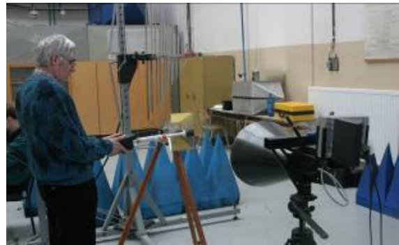
Fig.8. Calibration of calorimetric sensor
