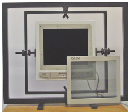
Fig. 2 Measured LCD display steady in the mechanical support.
