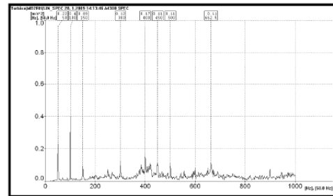
Fig. 5 Frequency spectrum of rms values of vibration acceleration
