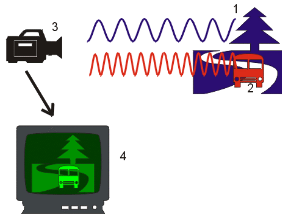
Fig.2 Principle of recording of thermal radiation of bodies in IR region
