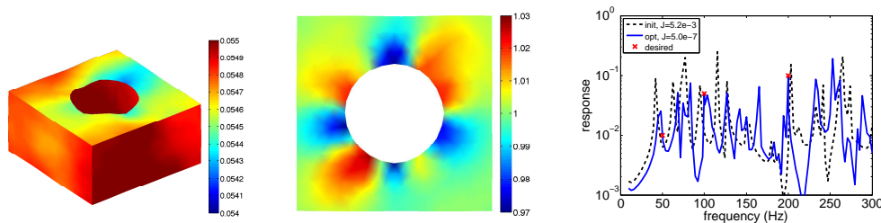
FIG. 2. The initial shape was a box with flat faces and uniform thickness of 0.05. Left plot: The optimized shape. Color indicates the shell thickness. Center plot: The top face. Color indicates shell height. Right plot: The transfer functions corresponding to the initial shape and the optimized shape, as well as the N_\omega = 3 frequencies with corresponding desired values r_k for the transfer function ( \times ).
