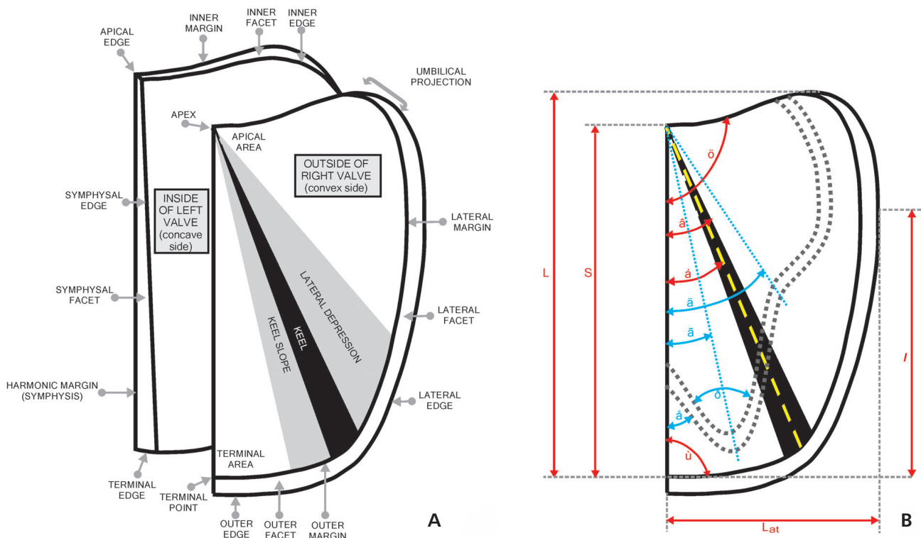
Figure 2. A – morphology of aptychi (modified from Trauth 1927, Arkell 1957, Gaşiorowski 1962b). • B – length and angular parameters measured on valves of ribbed aptychi, convex side of the right valve (modified from Gaşiorowski 1959).
