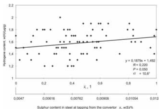
Figure 6: Dependence of hydrogen content on the sulphur content in steel during tapping from the converter
