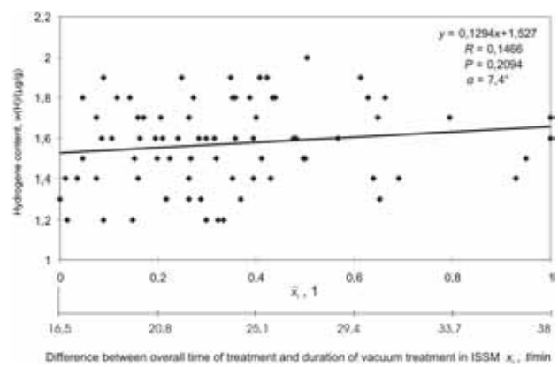
Figure 9: Dependence of the hydrogen content on the time when the steel is not vacuum treated in the ISSM
