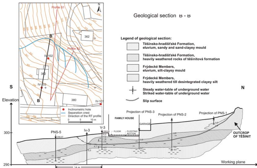
Fig. 3: Geological section and map of the interest area along with the sections placement
