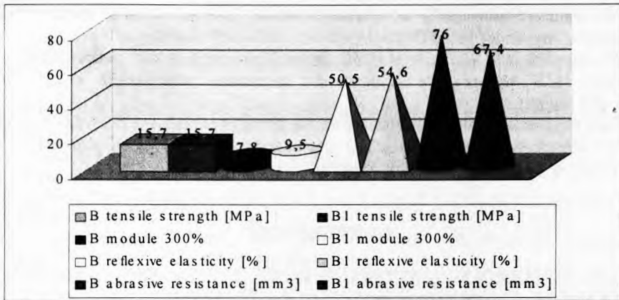
Graph 4: Tensile strength, module 300%, reflexive elasticity and abrasive resistance of sidewall compound without and with Werbablend H250.
