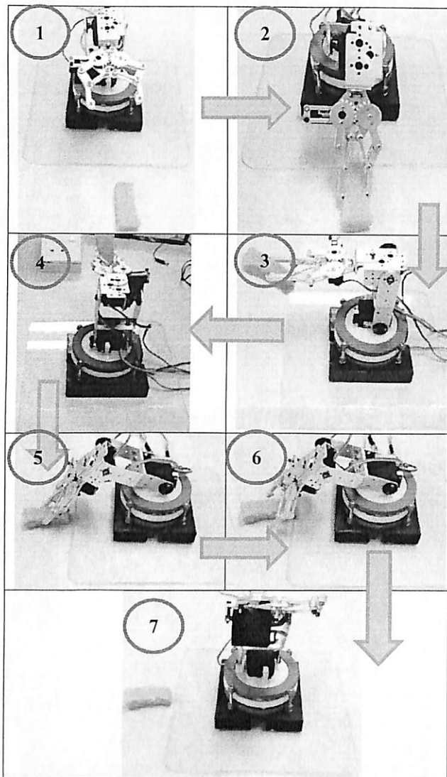
Figure 6: The robotic arm picks and place operation
