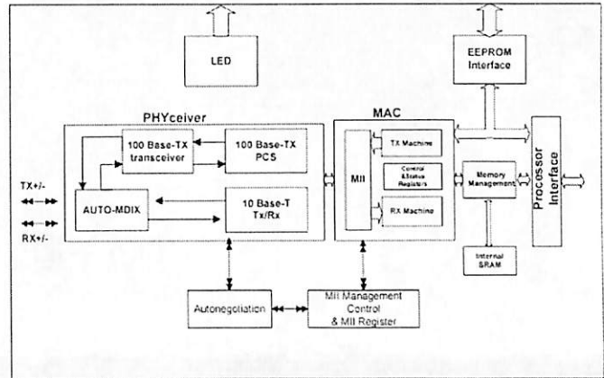
Figure 2: Block diagram of Ethernet controller DM9000A
