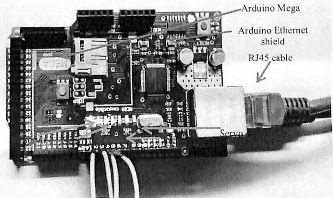
Figure 3: Hardware interface between Arduino Mega and Arduino Ethernet shield
