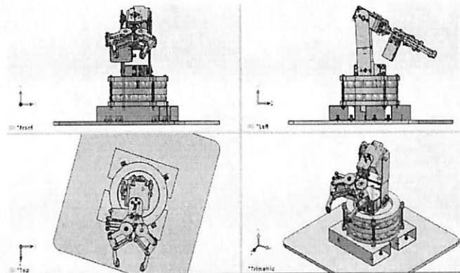
Figure 5: Combine view of the robotic arm
