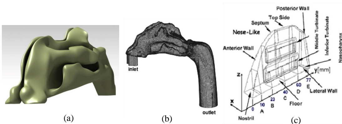
Figure 2.4: Models of the nasal cavity (a) Anatomically identical model, (b) Nasal cavity with additional inlet tube and extended nasopharynx, and (c) Simplified nose-like model (Figures obtained from (Shi et al., 2006) and (Elad et al., 2008))
