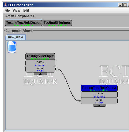
Figure 5 Graph editor
