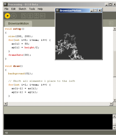
Figure 8 Processing IDE
