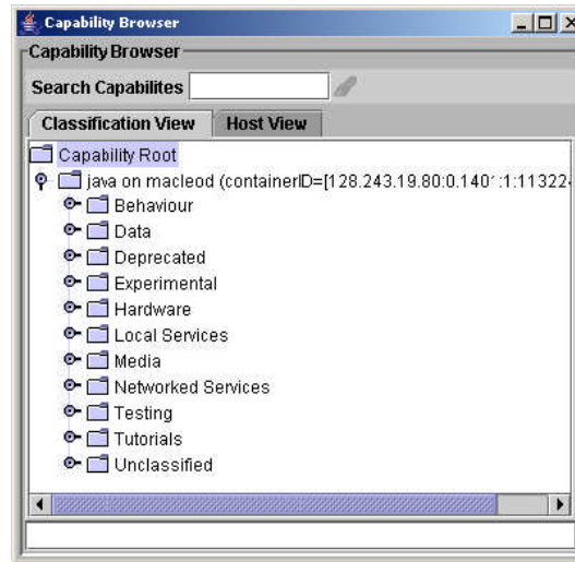
Figure 4 Capability browser
