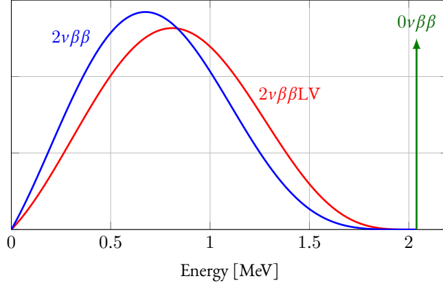
Figure 3: Energy spectra for different double-beta decay modes of ^{76}\text{Ge} : the two-neutrino mode (blue), the Lorentz violating mode (red), the neutrinoless mode (green).
