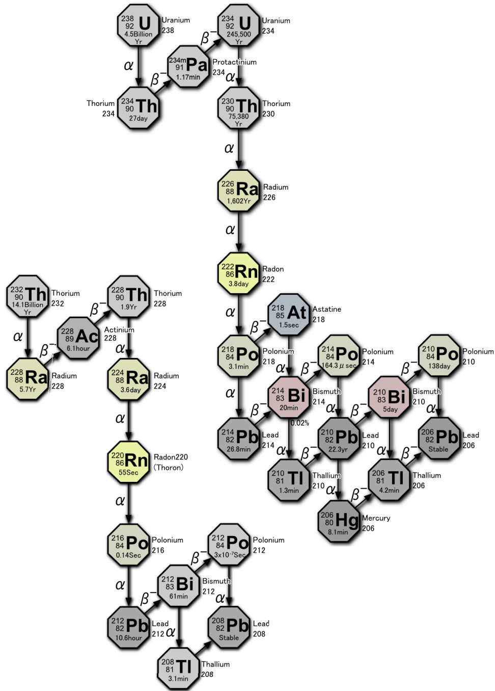
Figure 12: Schemes of ^{238}\text{U} and ^{232}\text{Th} decay chains.
