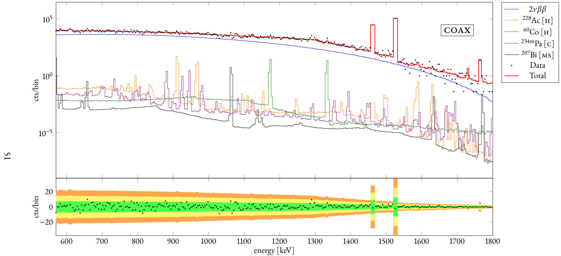
Figure 22: Part of the background decomposition in the range [570, 1800] keV for the summed enriched coaxial energy spectrum resulting from the minimal model with informative priors. The ratio between the counts and the bin width is plotted against the energy. The residuals, computed as the subtraction between the data and the total fitted curve, is also shown. Legend: [HOMLAR] = homogeneous in LAr, [F] = fiber-shroud, [H] = holder mounting, [MS] = mini-shroud, [C] = cables, [N + ] = n + -contact.
