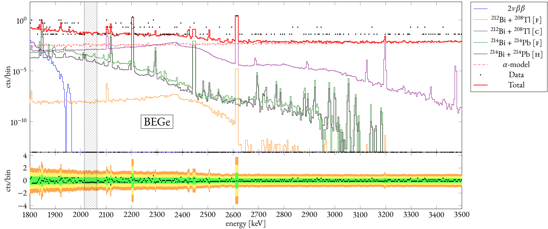
Figure 24: Part of the background decomposition in the range [1800, 3500] keV for the summed BEGe energy spectrum resulting from the minimal model with informative priors. The ratio between the counts and the bin width is plotted against the energy. The residuals, computed as the subtraction between the data and the total fitted curve, is also shown. Legend: [HOMLAR] = homogeneous in LAr, [F] = fiber-shroud, [H] = holder mounting, [MS] = mini-shroud, [C] = cables, [N + ] = n + -contact.
