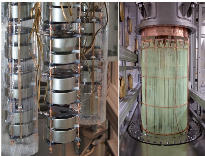
Figure 6: On the left: some detector strings — final integration in July 2015, photo courtesy of Bernhard Schwingenheuer. On the right: the fiber-shroud being deployed in LAr — November 2015, photo courtesy of Mark Heisel.
