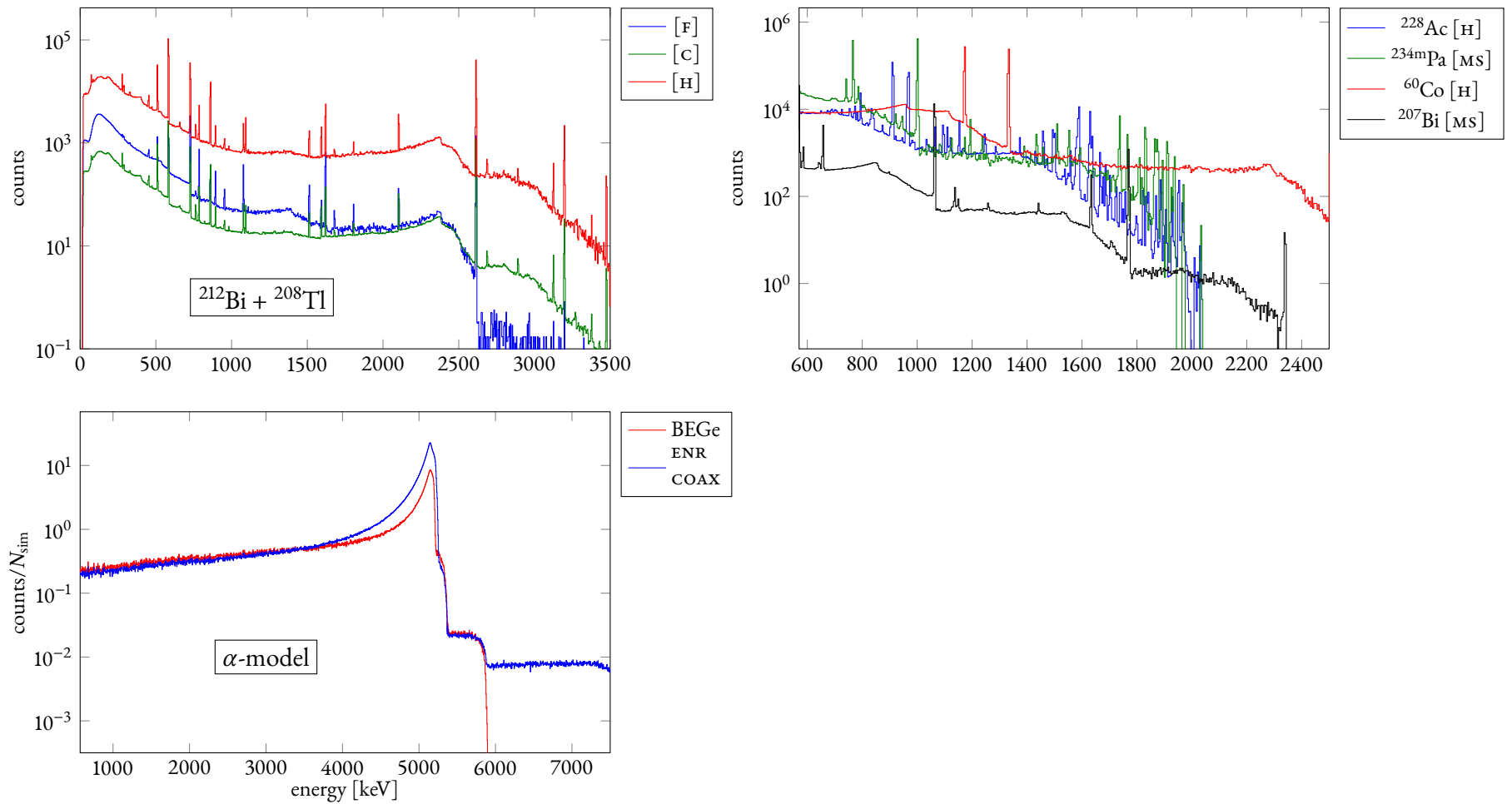
Figure 11: Simulated spectra, normalized to activity = 1 Bq/kg, as described in §4, except for the \alpha -model which is simply normalized to the number of generated events. All spectra refer to BEGe detectors. Legend: [MS] = mini-shroud, [C] = cables, [H] = holders, [F] = fiber-shroud. Top left: ^{212}\text{Bi} and ^{208}\text{Tl} summed spectra; top right: ^{60}\text{Co} , ^{228}\text{Ac} , ^{234\text{m}}\text{Pa} and ^{207}\text{Bi} ; bottom left: \alpha -model.
