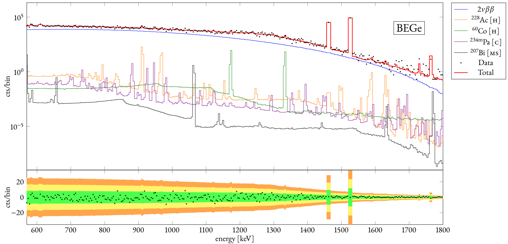
Figure 19: Part of the background decomposition in the range [570, 1800] keV for the summed BEGe energy spectrum resulting from the minimal model with informative priors. The ratio between the counts and the bin width is plotted against the energy. The residuals, computed as the subtraction between the data and the total fitted curve, is also shown. Legend: [HOMLAR] = homogeneous in LAR, [F] = fiber-shroud, [H] = holder mounting, [MS] = mini-shroud, [C] = cables, [N + ] = n + -contact.
