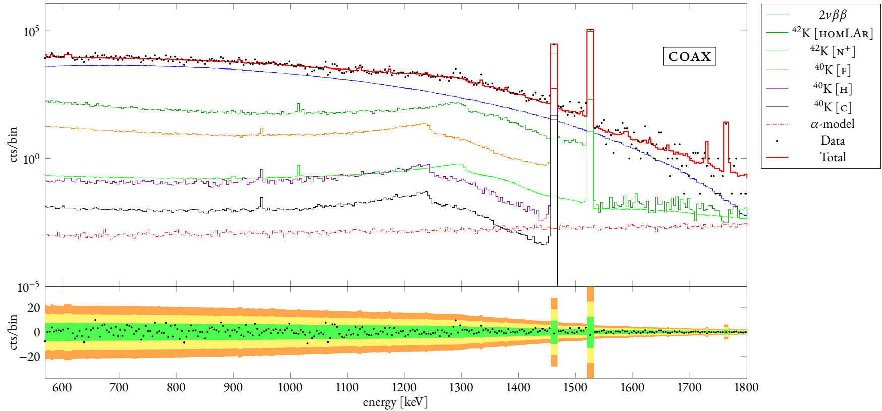
Figure 20: Part of the background decomposition in the range [570, 1800] keV for the summed enriched coaxial energy spectrum resulting from the minimal model with informative priors. The ratio between the counts and the bin width is plotted against the energy. The residuals, computed as the subtraction between the data and the total fitted curve, is also shown. Legend: [HOMLAR] = homogeneous in LAr, [F] = fiber-shroud, [H] = holder mounting, [MS] = mini-shroud, [C] = cables, [ \text{N}^+ ] = \text{n}^+ -contact.
