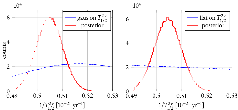
Figure 14: Prior and posterior distributions of 1/T_{1/2}^{2\nu} . On the right: result with a uniform prior in T_{1/2}^{2\nu} , on the left: result with a gaussian prior in T_{1/2}^{2\nu} centered on the GERDA Phase I result (35).
