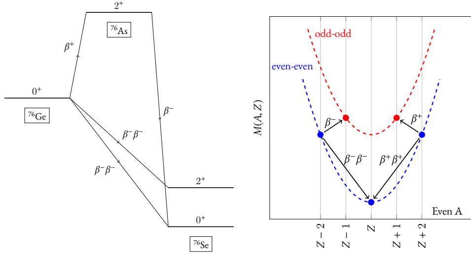
Figure 2: On the left: schematic illustration of the energy level structure of the 2\nu\beta^-\beta^- decay of ^{76}\text{Ge} into ^{76}\text{Se} . On the right: general energy level configuration for double-beta decay emitters. The situation for a nucleus with even mass number A is presented: the mass parabola, representing the dependence of the binding energy M(A, Z) on the atomic number Z , is plotted for even-even (even number of protons and neutrons) and odd-odd nuclei with the relevant \beta and \beta\beta decays among them.
