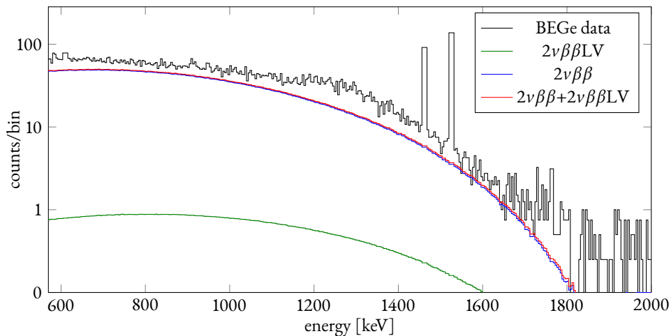
Figure 16: Double beta fitted spectra for the BEGe data set: the black histogram represents the data, the blue shape is the Standard Model double-beta decay mode, the green one is the Lorentz-violating mode with \hat{a}_{\text{of}}^{(3)} at 90% C.I. and the red one is the sum between the two modes.
