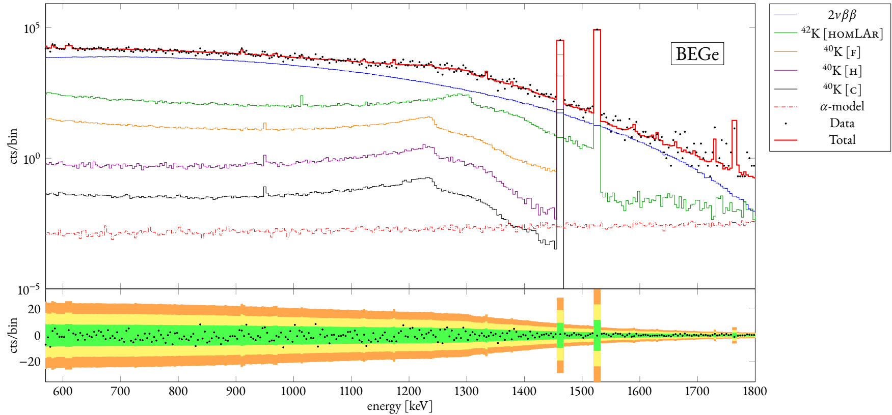
Figure 17: Part of the background decomposition in the range [570, 1800] keV for the summed BEGe energy spectrum resulting from the minimal model with informative priors. The ratio between the counts and the bin width is plotted against the energy. The residuals, computed as the subtraction between the data and the total fitted curve, is also shown. Legend: [HOMLAR] = homogeneous in LAr, [F] = fiber-shroud, [H] = holder mounting, [MS] = mini-shroud, [C] = cables, [N + ] = n + -contact.
