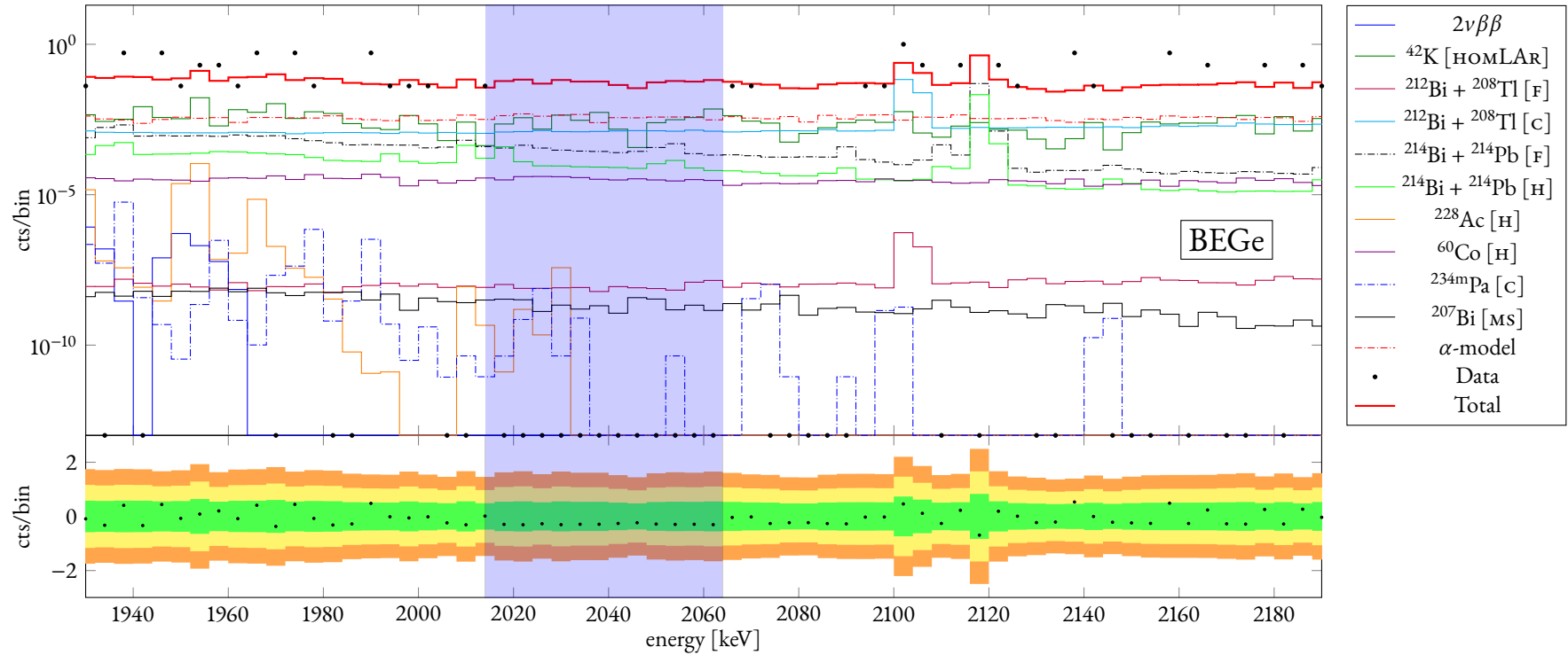
Figure 29: Background decomposition in the range [1930, 2190] keV (the ROI) for the summed BEGe energy spectrum resulting from the minimal model with informative priors. The ratio between the counts and the bin width is plotted against the energy. The residuals, computed as the subtraction between the data and the total fitted curve, is also shown. Legend: [HOMLAR] = homogeneous in LAr, [F] = fiber-shroud, [H] = holder mounting, [MS] = mini-shroud, [C] = cables, [N + ] = n + -contact.
