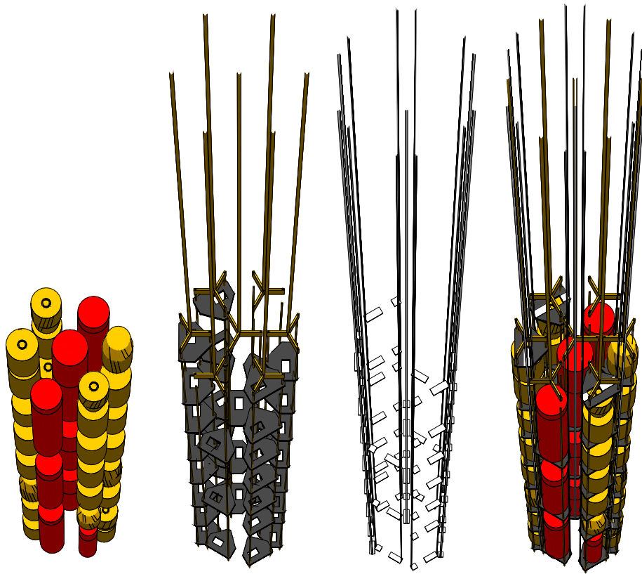
Figure 8: Implementation of the simulated volumes in MAGE. From left to right: the germanium detectors, the holder mounting, the cables and the three volumes put together.
