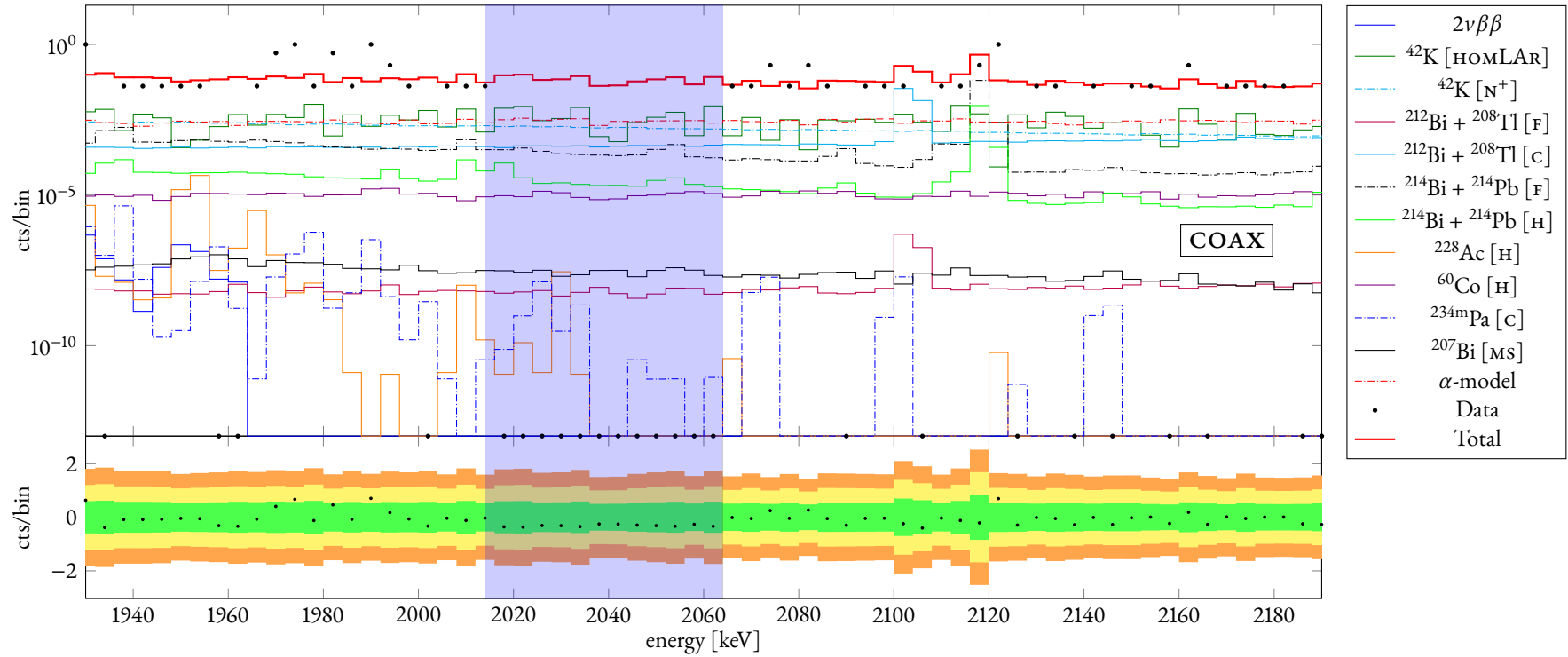
Figure 30: Background decomposition in the range [1930, 2190] keV (the ROI) for the summed enriched coaxial energy spectrum resulting from the minimal model with informative priors. The ratio between the counts and the bin width is plotted against the energy. The residuals, computed as the subtraction between the data and the total fitted curve, is also shown. Legend: [HOMLAR] = homogeneous in LAr, [F] = fiber-shroud, [H] = holder mounting, [MS] = mini-shroud, [C] = cables, [ \text{N}^+ ] = \text{n}^+ -contact.
