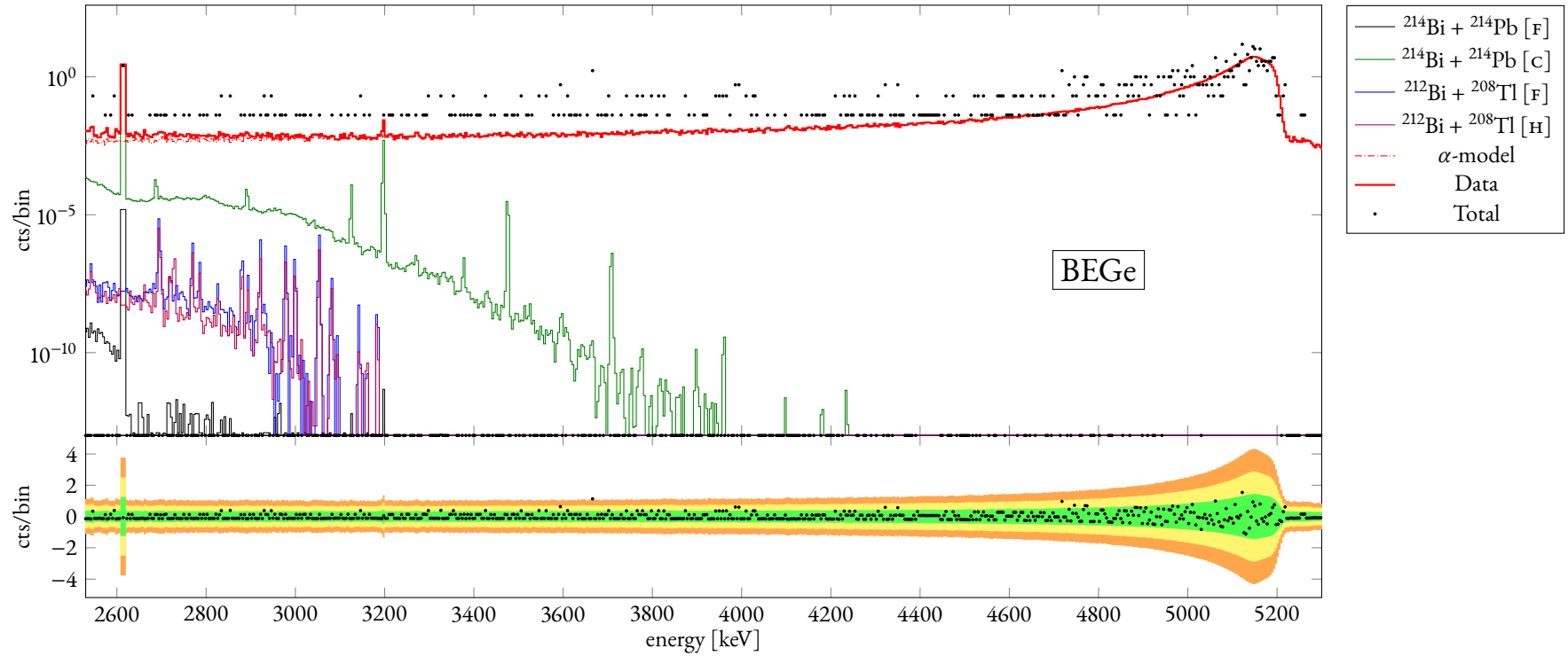
Figure 27: Part of the background decomposition in the range [2500, 5300] keV for the summed BEGe energy spectrum resulting from the minimal model with informative priors. The ratio between the counts and the bin width is plotted against the energy. The residuals, computed as the subtraction between the data and the total fitted curve, is also shown. Legend: [HOMLAR] = homogeneous in LAr, [F] = fiber-shroud, [H] = holder mounting, [MS] = mini-shroud, [C] = cables, [N + ] = n + -contact.
