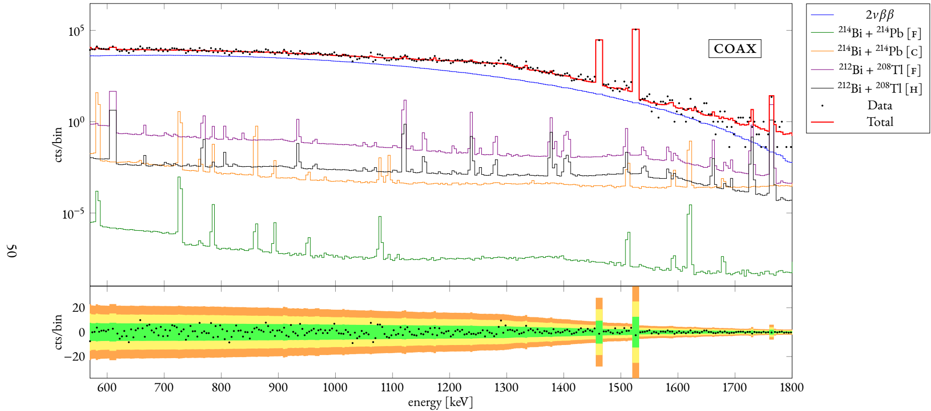
Figure 21: Part of the background decomposition in the range [570, 1800] keV for the summed enriched coaxial energy spectrum resulting from the minimal model with informative priors. The ratio between the counts and the bin width is plotted against the energy. The residuals, computed as the subtraction between the data and the total fitted curve, is also shown. Legend: [HOMLAR] = homogeneous in LAr, [F] = fiber-shroud, [H] = holder mounting, [MS] = mini-shroud, [C] = cables, [N + ] = n + -contact.
