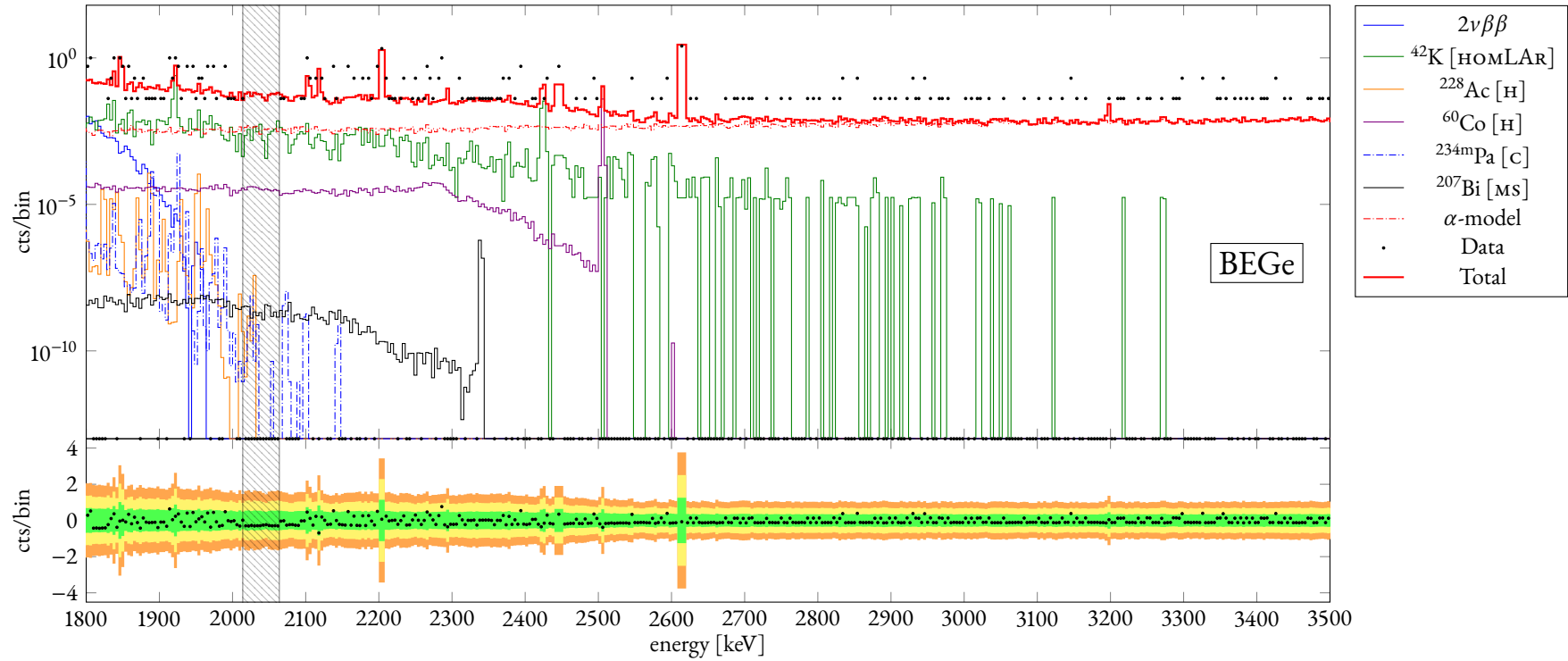
Figure 23: Part of the background decomposition in the range [1800, 3500] keV for the summed BEGe energy spectrum resulting from the minimal model with informative priors. The ratio between the counts and the bin width is plotted against the energy. The residuals, computed as the subtraction between the data and the total fitted curve, is also shown. Legend: [HOMLAR] = homogeneous in LAr, [F] = fiber-shroud, [H] = holder mounting, [MS] = mini-shroud, [C] = cables, [ \text{N}^+ ] = \text{n}^+ -contact.
