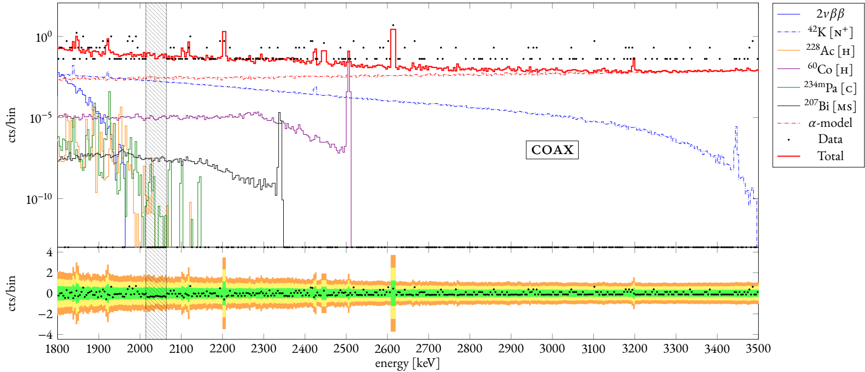
Figure 25: Part of the background decomposition in the range [1800, 3500] keV for the summed enriched coaxial energy spectrum resulting from the minimal model with informative priors. The ratio between the counts and the bin width is plotted against the energy. The residuals, computed as the subtraction between the data and the total fitted curve, is also shown. Legend: [HOMLAR] = homogeneous in LAr, [F] = fiber-shroud, [H] = holder mounting, [MS] = mini-shroud, [C] = cables, [N + ] = n + -contact.
