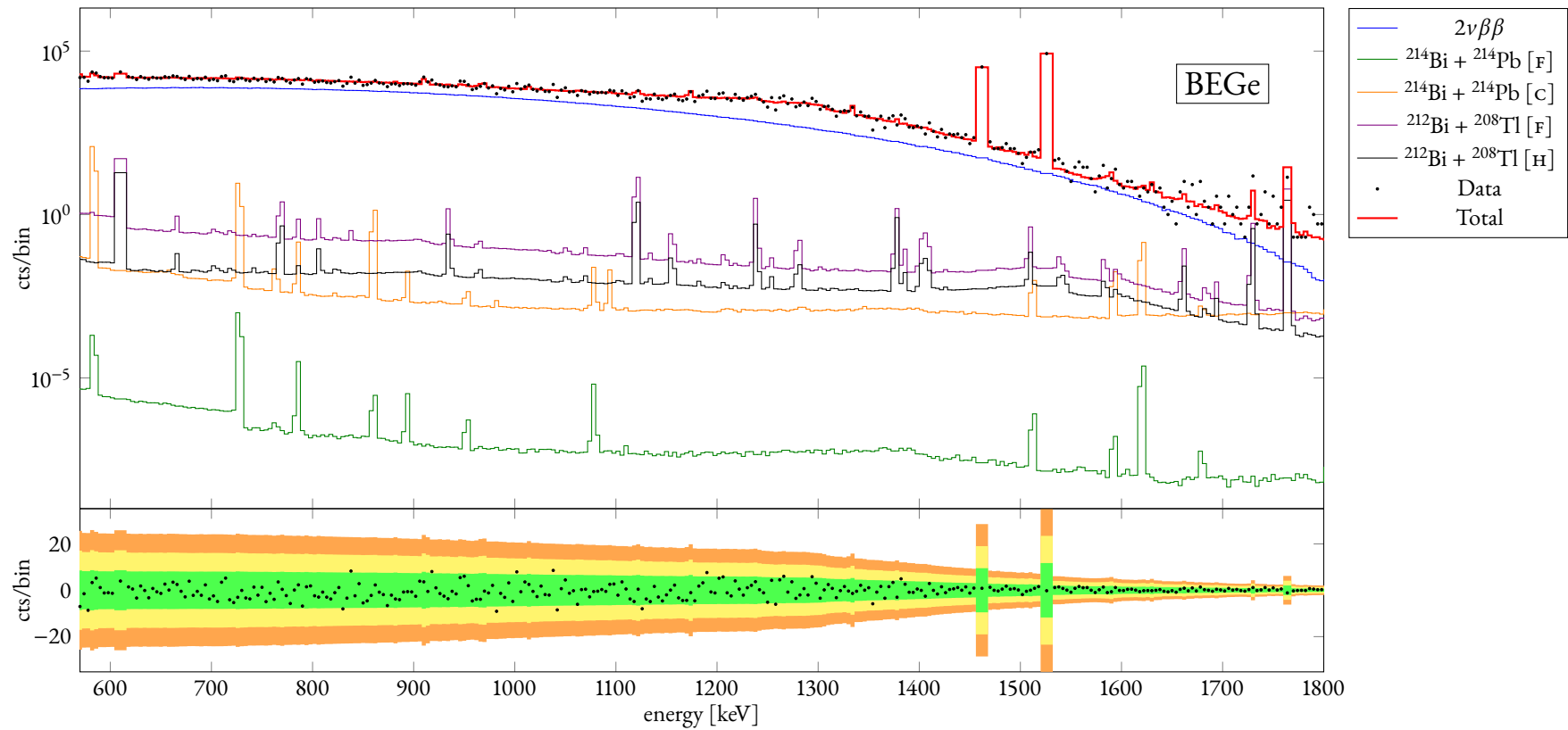
Figure 18: Part of the background decomposition in the range [570, 1800] keV for the summed BEGe energy spectrum resulting from the minimal model with informative priors. The ratio between the counts and the bin width is plotted against the energy. The residuals, computed as the subtraction between the data and the total fitted curve, is also shown. Legend: [HOMLAR] = homogeneous in LAr, [F] = fiber-shroud, [H] = holder mounting, [MS] = mini-shroud, [C] = cables, [N + ] = n + -contact.
