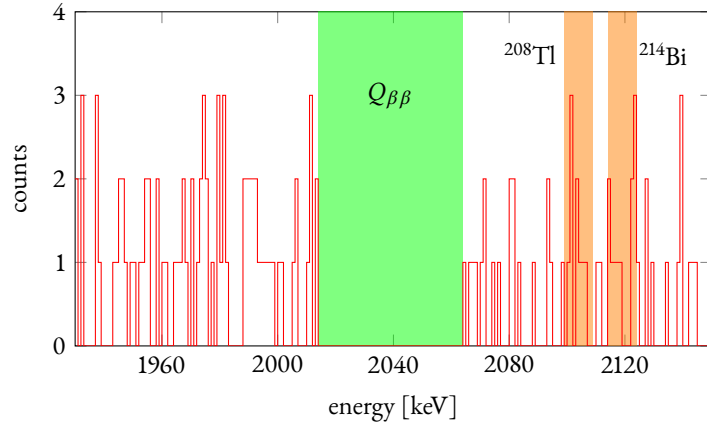
Figure 7: Energy window used to compute the background index, a 50 keV wide energy window around Q_{\beta\beta} and two 10 keV wide energy windows around the ^{208}\text{Tl} and ^{214}\text{Bi} peaks are excluded. The displayed data corresponds to the whole GERDA data set.
