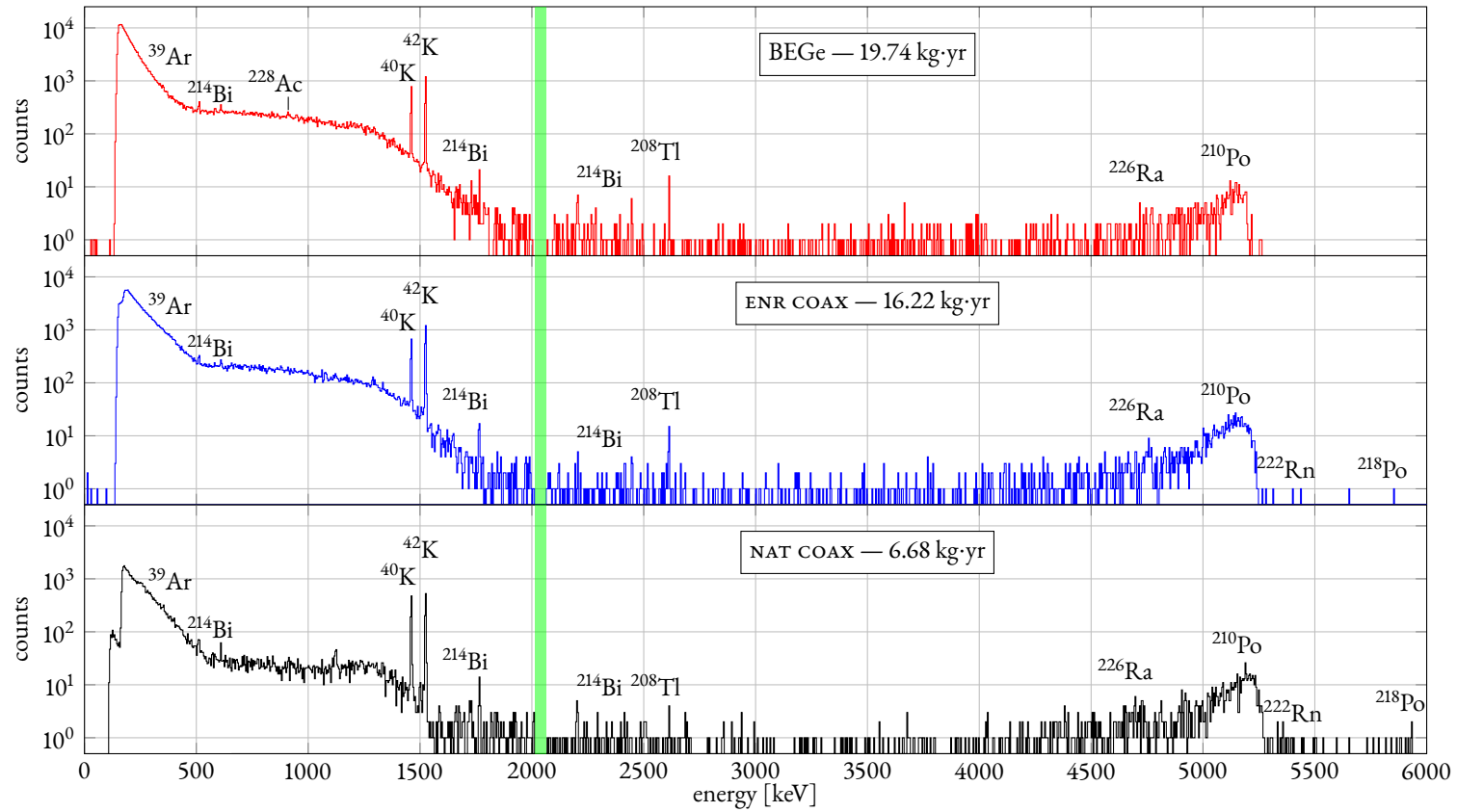
Figure 9: The summed energy spectrum (counts in logarithmic scale), showed separately for BEGe, enriched coaxial and natural coaxial detectors, produced using data from GERDA Phase II. The isotopes responsible for the relevant lines are reported on the plots together with the exposure. All the counts with energy greater than 3 MeV can be associated to \alpha -events on the p^+ electrode. The blinding window [Q_{\beta\beta} - 25 \text{ keV}, Q_{\beta\beta} + 25 \text{ keV}] is also shown in green. A 4 keV binning is adopted.
