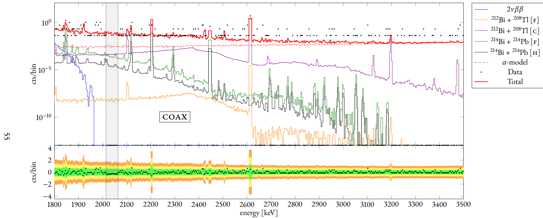
Figure 26: Part of the background decomposition in the range [1800, 3500] keV for the summed enriched coaxial energy spectrum resulting from the minimal model with informative priors. The ratio between the counts and the bin width is plotted against the energy. The residuals, computed as the subtraction between the data and the total fitted curve, is also shown. Legend: [HOMLAR] = homogeneous in LAr, [F] = fiber-shroud, [H] = holder mounting, [MS] = mini-shroud, [C] = cables, [N + ] = n + -contact.
