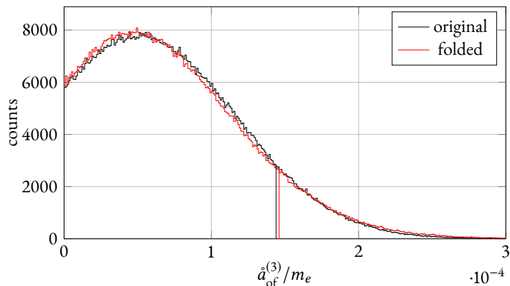
Figure 15: Posterior distribution of \hat{a}_{\text{of}}^{(3)} (in units of electron mass) before and after folding with the systematic uncertainty distribution.
