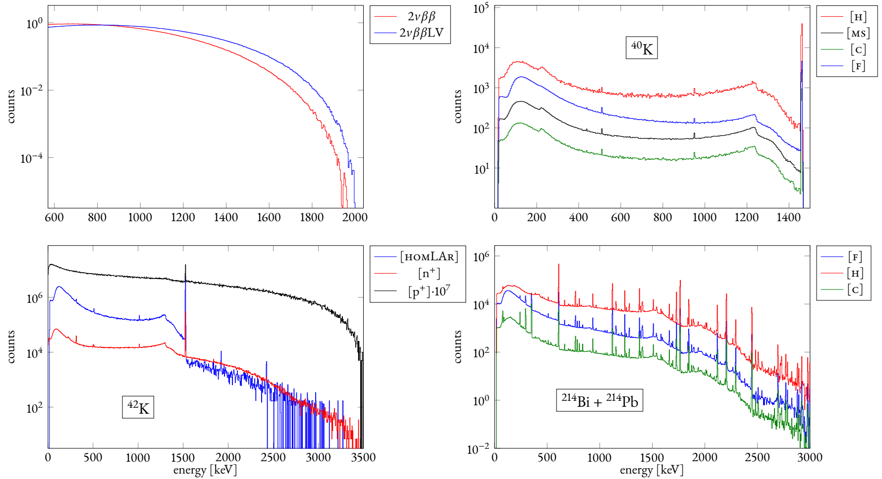
Figure 10: Simulated spectra, normalized to activity = 1 Bq/kg (except for 2\nu\beta\beta ), as described in §4. All spectra refer to BEGe detectors. Legend: [MS] = mini-shroud, [C] = cables, [H] = holders, [F] = fiber-shroud, [HOMLAR] = homogeneous in LAr, [ n^+ ]/[ p^+ ] = contacts. Top left: the Standard Model and Lorentz-violating double-beta decay modes; top right: ^{40}\text{K} ; bottom left: ^{42}\text{K} ; bottom right: ^{214}\text{Bi} and ^{214}\text{Pb} summed spectra.
