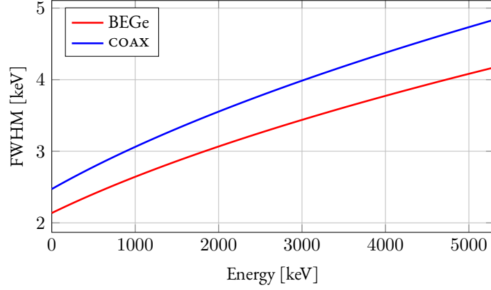
Figure 13: Combined resolution curves for the BEGes (red) and enriched coaxials (blue) detectors.
