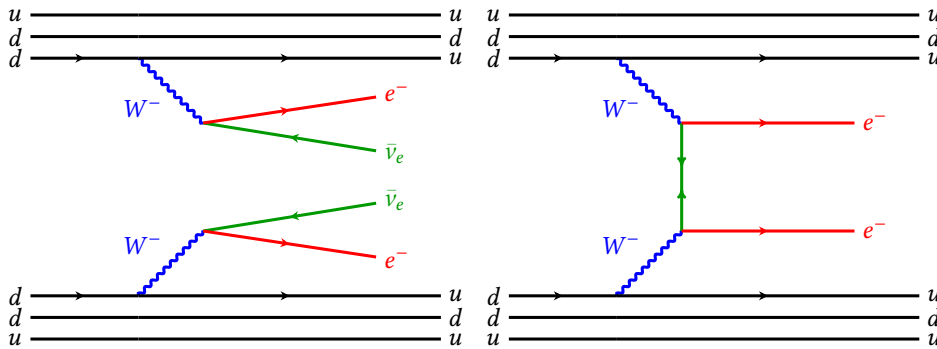
Figure 1: Feynman graphs for two-neutrino (left) and neutrinoless (right) double-beta decay.
