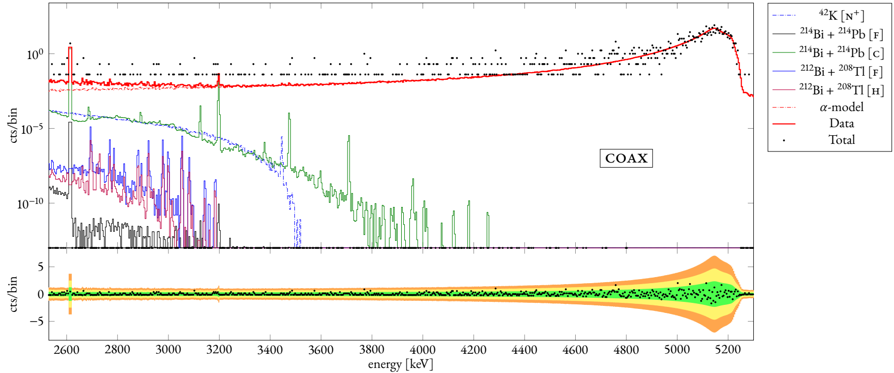
Figure 28: Part of the background decomposition in the range [2500, 5300] keV for the summed enriched coaxial energy spectrum resulting from the minimal model with informative priors. The ratio between the counts and the bin width is plotted against the energy. The residuals, computed as the subtraction between the data and the total fitted curve, is also shown. Legend: [HOMLAR] = homogeneous in LAr, [F] = fiber-shroud, [H] = holder mounting, [MS] = mini-shroud, [C] = cables, [ \text{N}^+ ] = \text{n}^+ -contact.
