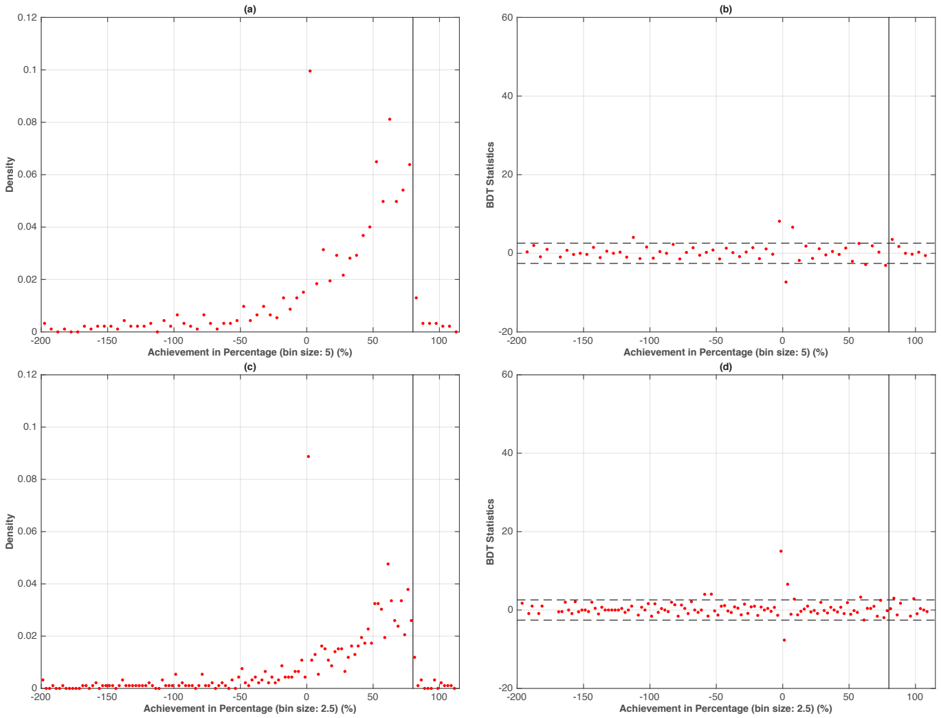
Figure A3. Probability distribution and the BDT test for energy saving achievement in percentage of non-compliant firms under the Top 10,000 Enterprises Program in 2014.
