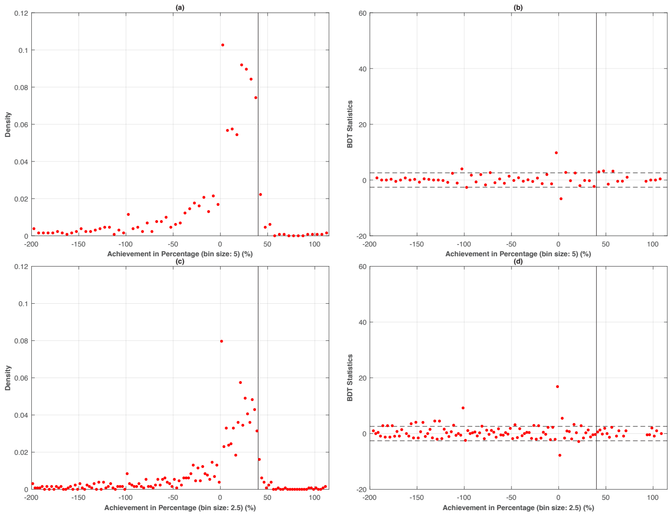
Figure A1. Probability distribution and the BDT test for energy saving achievement in percentage of non-compliant firms under the Top 10,000 Enterprises Program in 2012.
