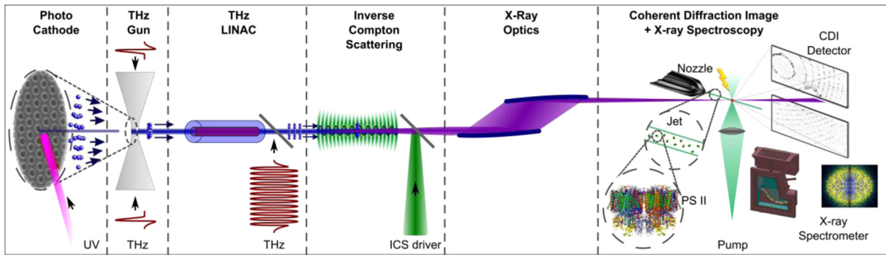
Fig. 2. Schematic layout of the AXSIS setup currently under construction at the SINBAD-facility at DESY in Hamburg.
