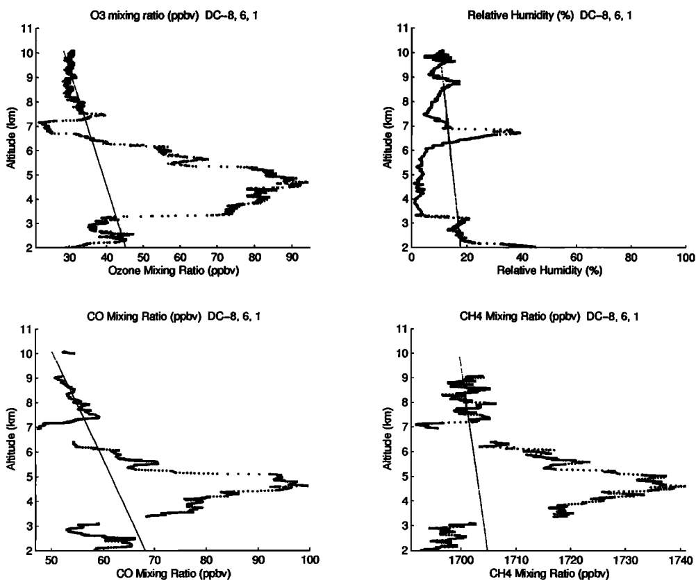
Figure 5. Vertical profiles of O_3 , CO, CH_4 , and H_2O , sampled during PEM-Tropics A DC-8 mission 6 (September 5, 1996) around 2145 UT, near 155^\circ W , and 15.5^\circ S . Thin lines are background levels as estimated by the new mode-based method.
