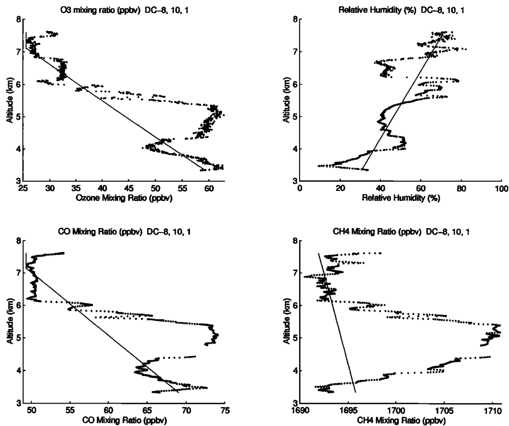
Figure 4. Vertical profiles of O_3 , CO, CH_4 , H_2O , and CO_2 , sampled during PEM-Tropics A DC-8 mission 10 (September 14, 1996) around 2305 UT, near 144.6^\circ W , 18.4^\circ S . Thin lines are background levels as estimated by the new mode-based method.
