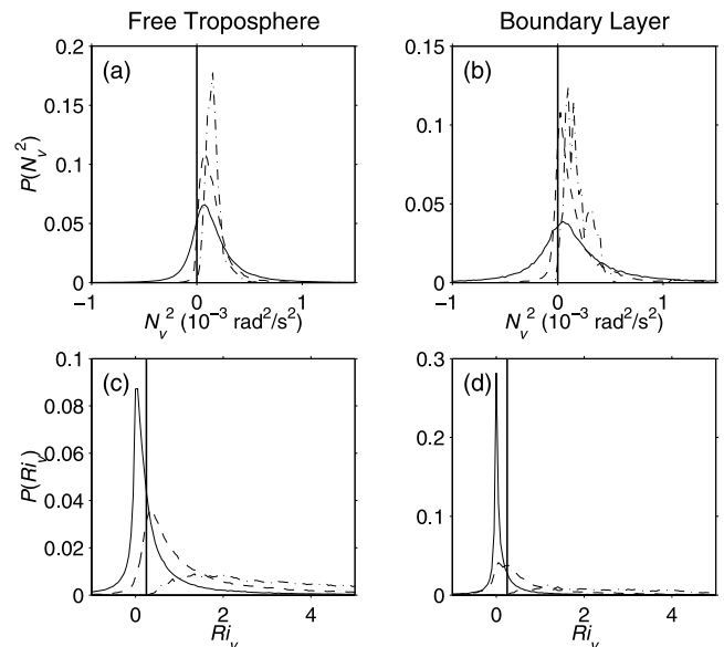
Figure 6. PDFs of N_v^2 and Ri_v for \Delta z = 10 \text{ m} (solid), 100 \text{ m} (dashed), and 1000 \text{ m} (dash-dotted). The left-hand column is for free tropospheric data and the right-hand column is for boundary layer data. The vertical lines in (a) and (b) mark N_v^2 = 0 . The vertical lines in (c) and (d) mark the critical Ri_v = 1/4 level.
