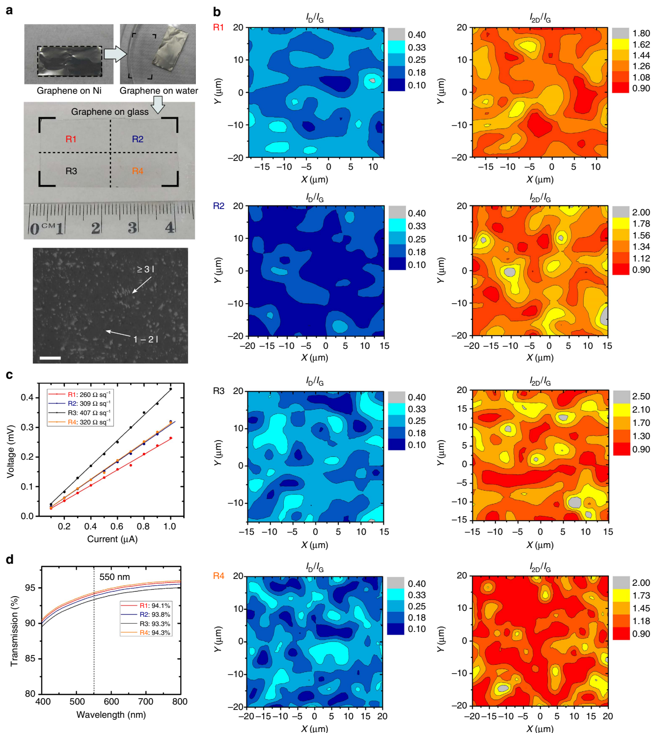
Figure 3 | Characterizations of the graphene film grown in an ambient-air environment. (a) A 4 × 2 cm 2 graphene grown on Ni foil is transferred onto glass. Measurements were taken over four quadrants as labelled on the graphene surface. An optical micrograph of the graphene film transferred onto glass is also included. (b) Raman spectral analyses of the intensity ratios of I_D/I_G and I_{2D}/I_G . (c) Four-point probe and (d) optical transmission measurements of sheet resistance of graphene films in the respective regions. Scale bar, 20 μm in a.
