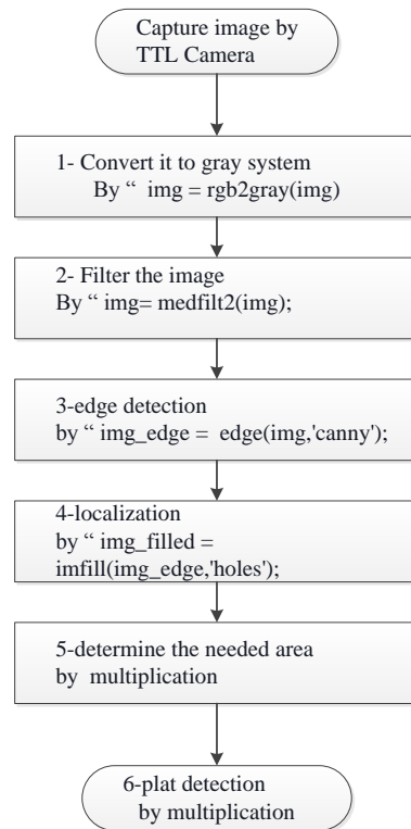
Fig. 1. Basic steps of plate detection.
