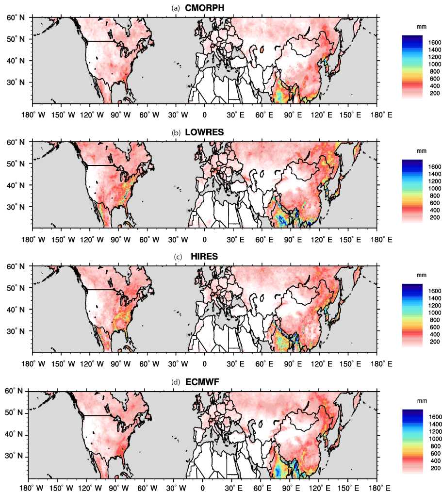
Figure 15. The 2-month accumulated precipitation. Panel (a) shows the CMORPH analysis, (b) shows the LOWRES simulation, and (c) displays the HIRES simulation. Panel (d) displays the accumulated precipitation from the operational ECMWF 12 h forecast starting at 00:00 and 12:00 UTC on each day.
