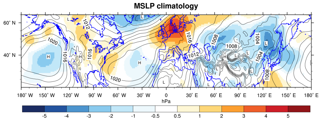
Figure 4. Mean sea level pressure climatology for July and August 2013 (black solid lines) from ERA-Interim. The shaded areas show the anomaly during July and August 2013 compared to the period 1979–2012.
