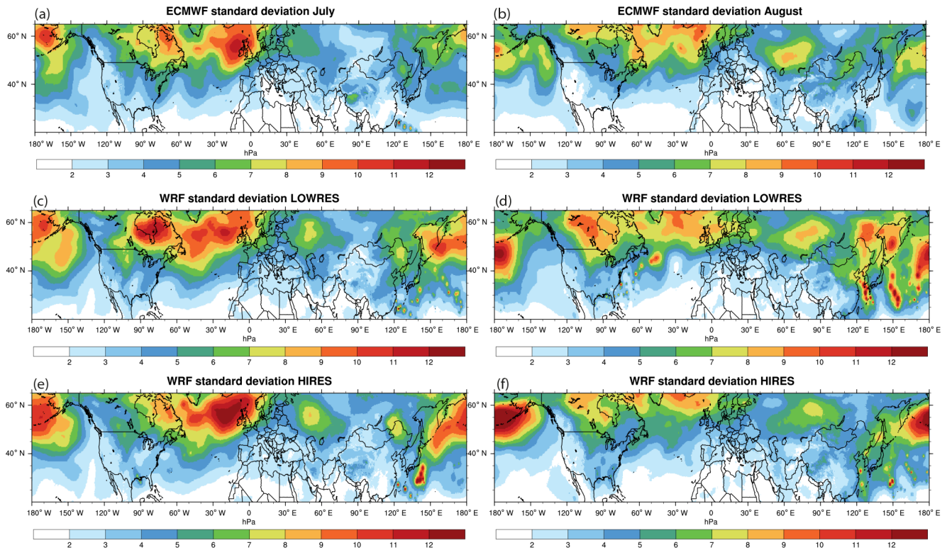
Figure 7. Mean sea level pressure standard deviation at 12:00 UTC for July 2013 (a, c, e) and August 2013 (b, d, f). The top row shows the ECMWF analysis, the middle row shows the LOWRES simulation, and the bottom row displays the HIRES simulation.
