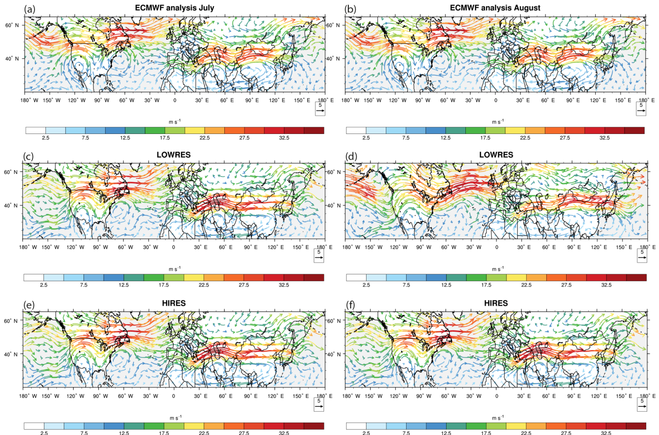
Figure 8. Mean 300 hPa wind velocities for July 2013 (a, c, e) and August 2013 (b, d, f). The top row shows the ECMWF analysis, the middle row shows the LOWRES simulation, and the bottom row displays the HIRES simulation.
