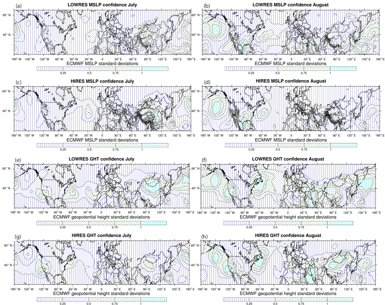
Figure 6. Model biases expressed in absolute terms of 2 ECMWF standard deviations for the LOWRES simulation (a, b, e, f) and the HIRES simulation (c, d, g, h) for the 12:00 UTC time steps. Left column: July 2013. Right column: August 2013. First two rows: mean sea level pressure. Bottom two rows: 500 hPa geopotential height.
