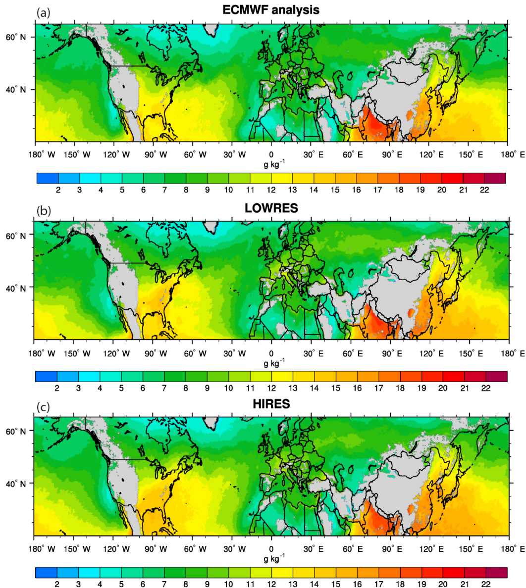
Figure 11. Average 925 hPa water vapor mixing ratio for 12:00 UTC of the ECMWF analysis (a) and the LOWRES simulation (b). The bottom panel shows the HIRES simulation.
