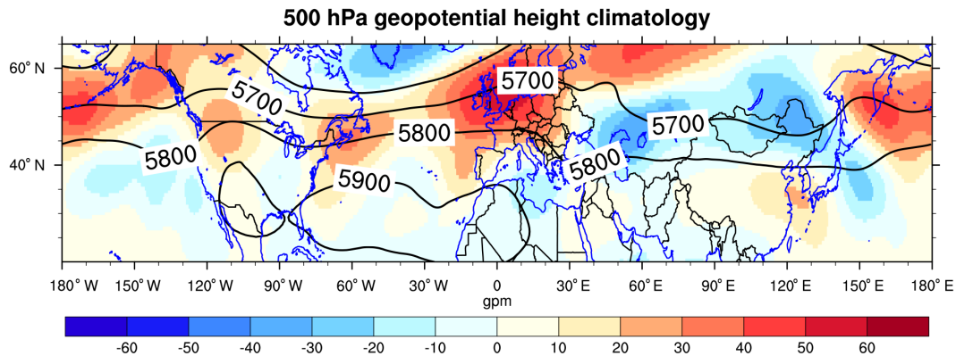
Figure 2. ERA-Interim 500 hPa geopotential height climatology for July and August 2013 (black solid lines). The shaded areas show the anomaly during July and August 2013 compared to the period 1979–2012.
