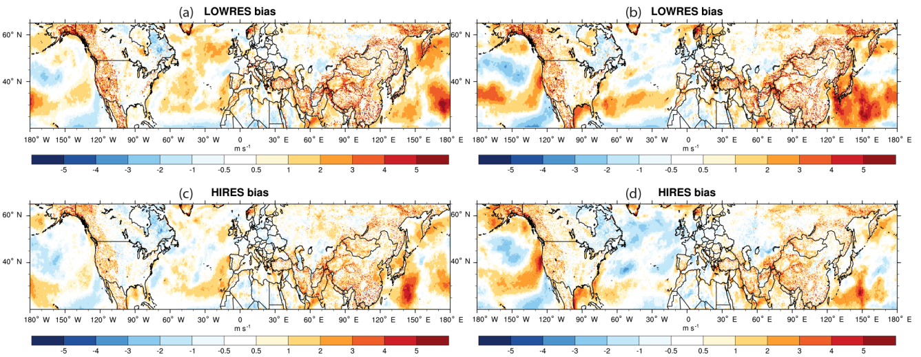
Figure 14. The 10 m wind speed bias in July (a, c) and August 2013 (b, d) for the LOWRES simulation (a, b) and the HIRES simulation (c, d).
