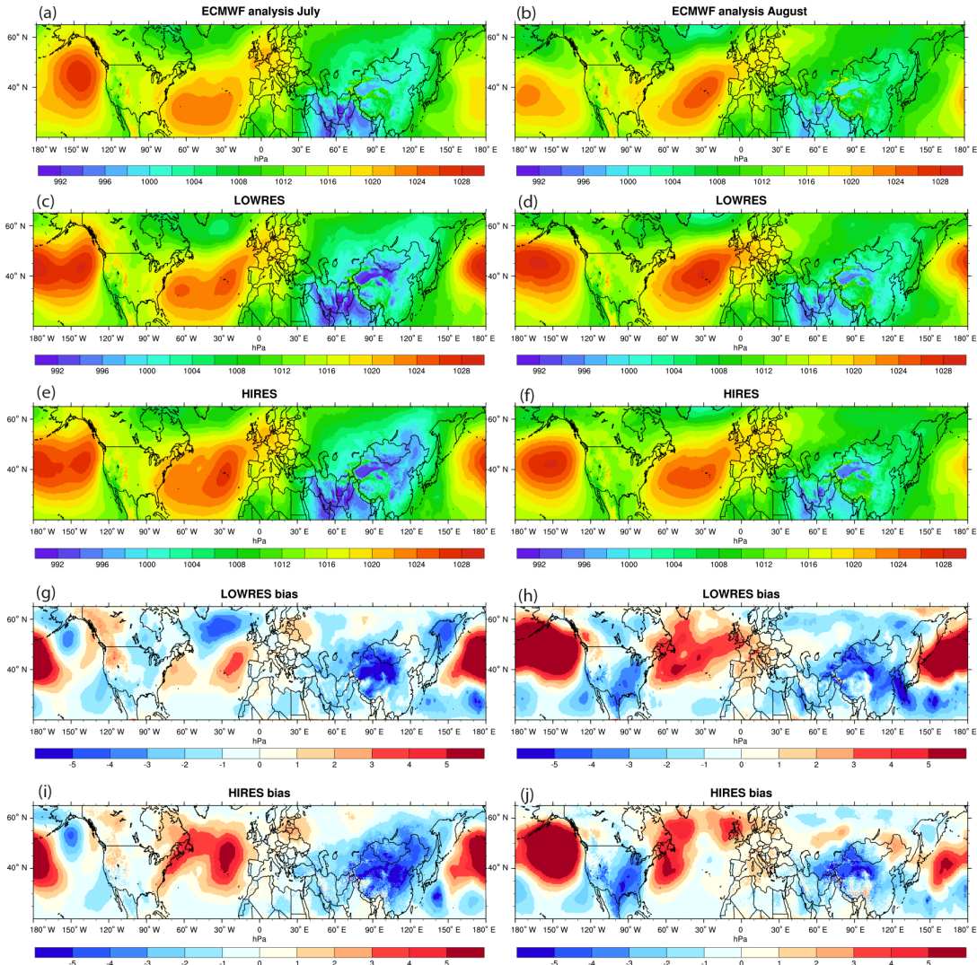
Figure 5. Average mean sea level pressure and mean difference between the WRF simulations and ECMWF analysis at the 12:00 UTC time steps for July 2013 and August 2013. The first row shows the ECMWF analysis (a, b) followed by the LOWRES simulation (c, d) and the HIRES simulation (e, f). The two lowermost rows show the mean bias for the LOWRES (g, h) and the HIRES simulations (i, j) compared to the ECMWF analysis for the two different months.
