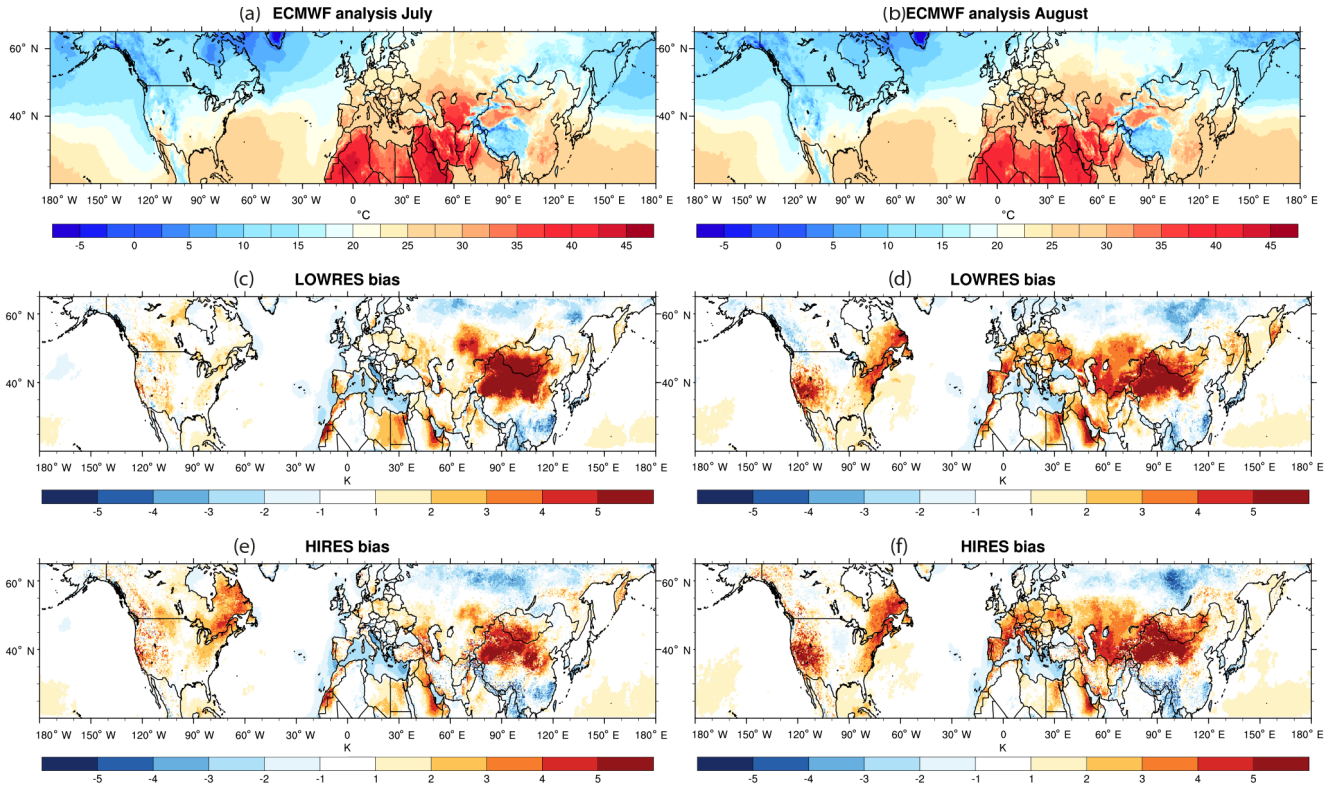
Figure 13. Mean 2 m temperature at 12:00 UTC in July (a, c, e) and August (b, d, f). The top row shows the ECMWF analysis, the middle row displays the LOWRES simulation, and the bottom row represents the HIRES simulation. Reddish colors indicate a warm bias of the WRF simulations.
