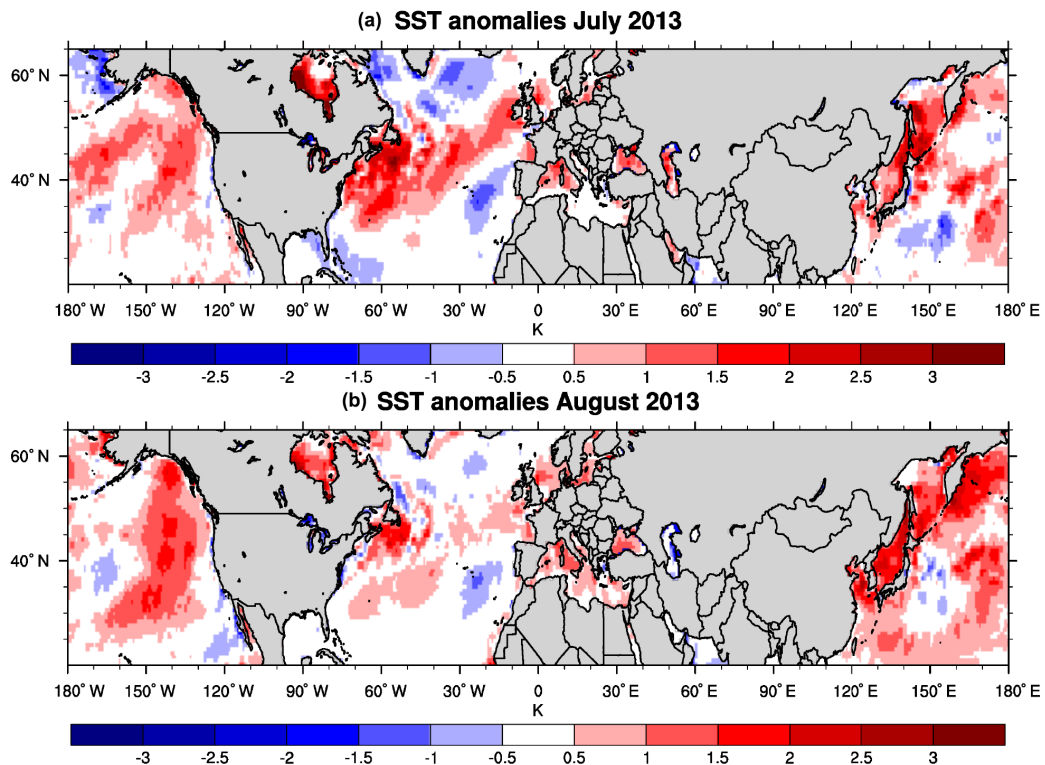
Figure 3. ERA-Interim sea surface temperature (SST) anomalies in July 2013 (a) and August 2013 (b) compared to the climatological period 1979–2012.
