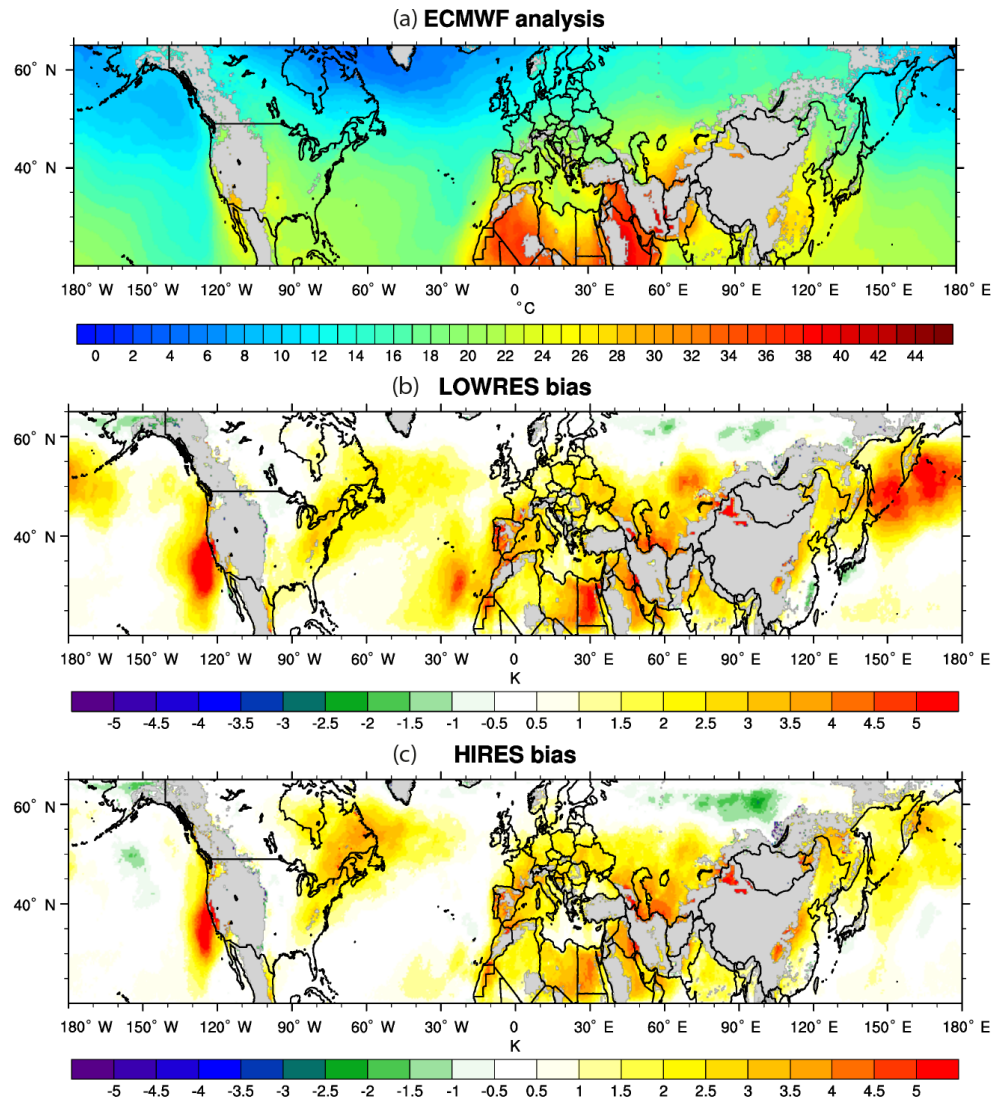
Figure 12. Mean 925 hPa temperature for 12:00 UTC of the ECMWF analysis (a). Panels (b) and (c) show the deviation of the LOWRES and HIRES simulations from the ECMWF analysis, respectively.
