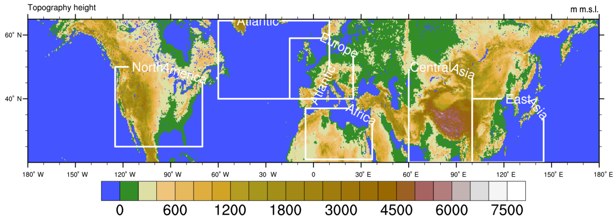
Figure 1. Model domain of the latitude-belt simulation. The white rectangles denote the domains used for verification of precipitation.
