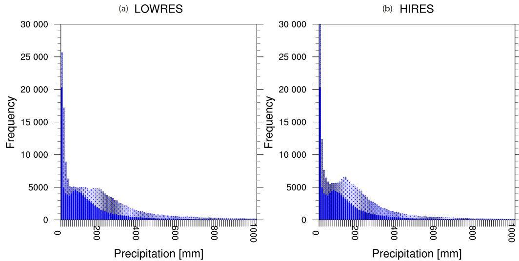
Figure 16. Histogram of the 2-month accumulated precipitation by using the CMORPH data over land points only. The filled blue bars denote the CMORPH data set and the cross-hatched bars denote the LOWRES (a) and HIREs simulation data (b).
