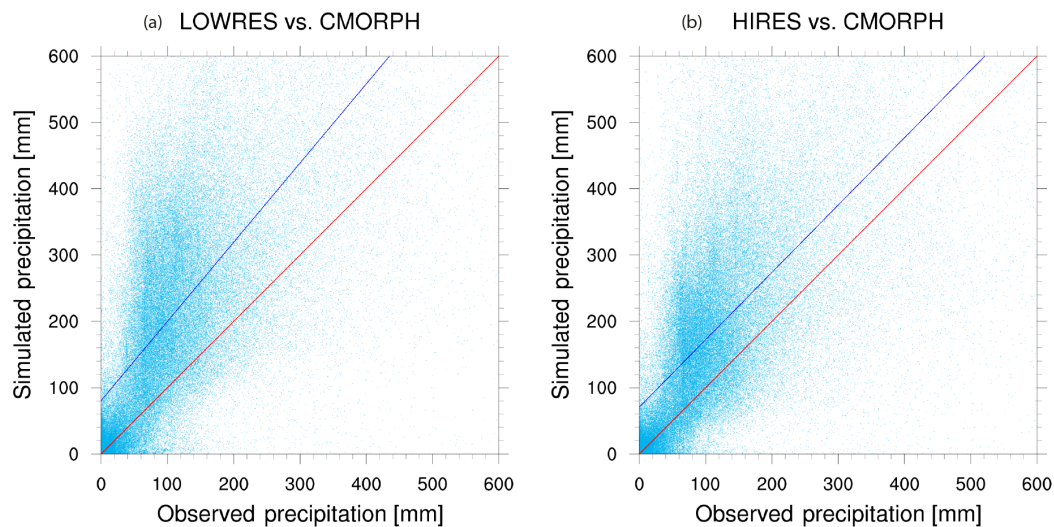
Figure 17. Scatter plot of the accumulated precipitation over the 2-month period including regression lines. The left panel shows the LOWRES simulation versus the CMORPH data. The red line indicates the perfect result. The right panel shows the HIREs simulation versus the CMORPH data.
