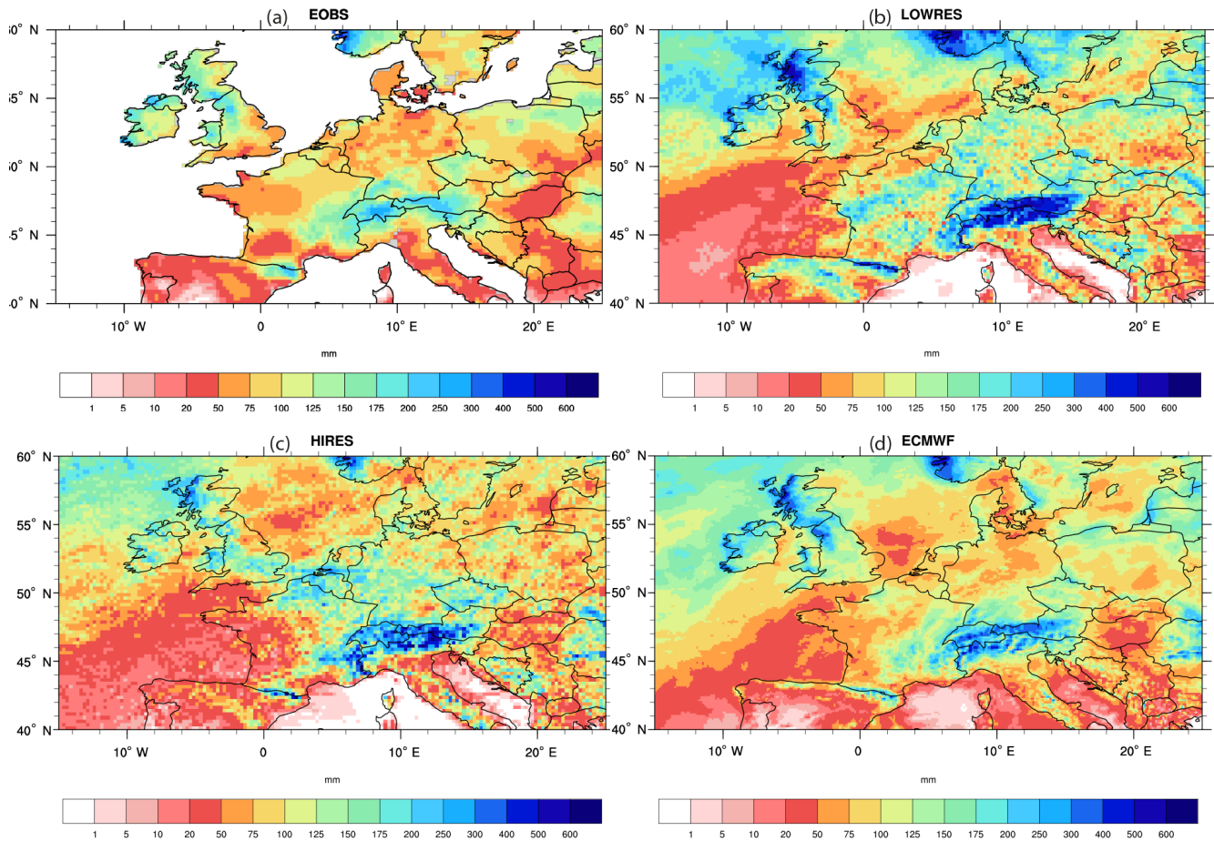
Figure 18. The 2-month accumulated precipitation over Europe. Panel (a) shows the E-OBS data set, (b) shows the LOWRES simulation, (c) displays the HIRES simulation, and (d) shows the ECMWF forecast.
