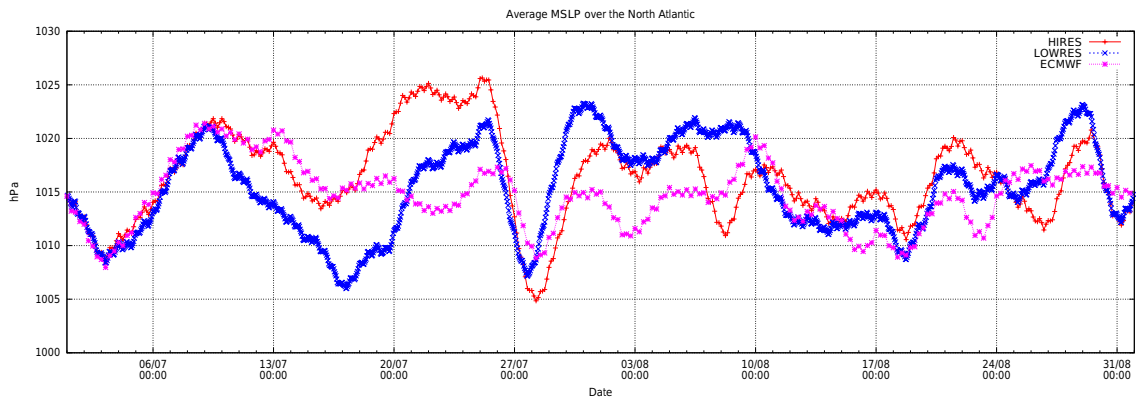
Figure 10. Time series of the MSLP averaged between 40 and 65° N, and 60° W and 10° E.
