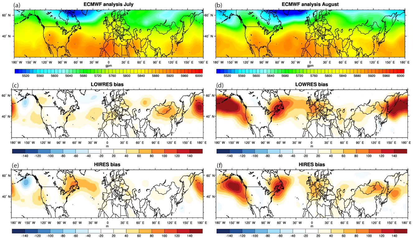
Figure 9. Mean 500 hPa geopotential height and mean differences between the WRF simulations and ECMWF analysis at the 12:00 UTC time steps for July 2013 (a, c, e) and August 2013 (b, d, f). The top row shows the ECMWF analysis, the middle row shows the LOWRES simulation, and the bottom row displays the HIRES simulations.
