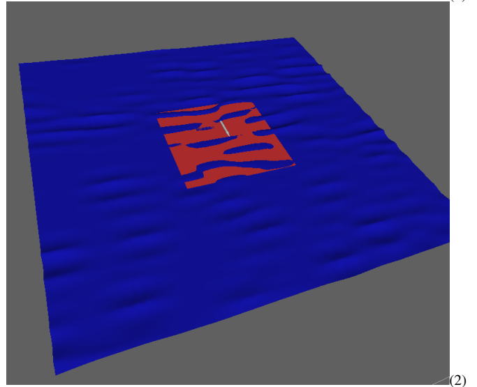
Two single wave group maps with the same wave number k = 0.2 \text{ rad m}^{-1} and the same envelope extension \varrho = 3 * \pi/k . The surface S of the red squares (at level z = 0 ) is such that \lambda_1/S = 1 (up) while \lambda_2/S = 4 (down). The average steepnesses at the center of the groups of these maps are \sigma_1 k = \pi \cdot 0.06 and \sigma_2 k = \pi \cdot 0.03 . Since \lambda_1 \sigma_1^2 = \lambda_2 \sigma_2^2 , both blue sea-surfaces ( 500 \text{ m} \times 500 \text{ m} ) present the same map spectrum.
