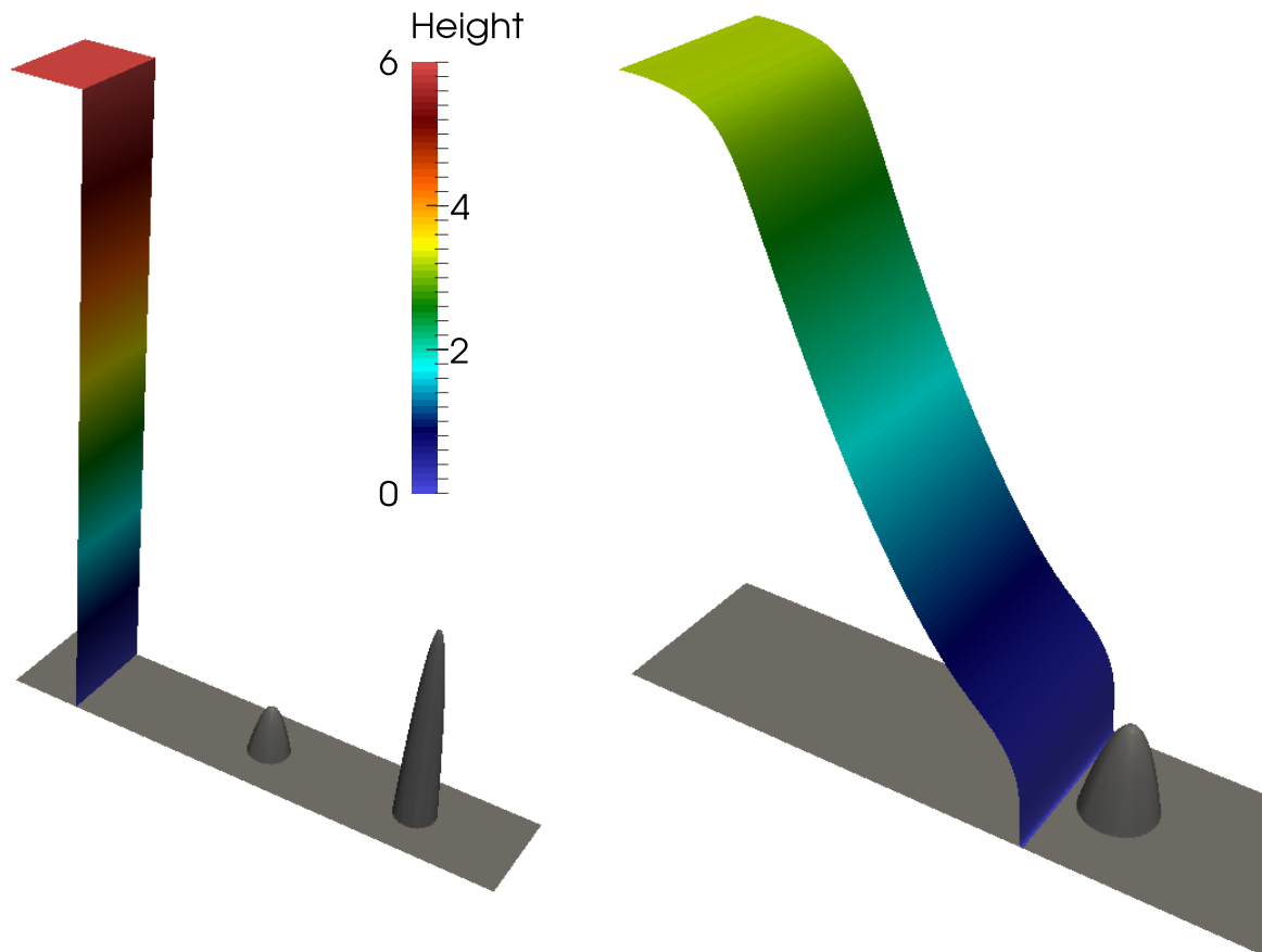
Figure 4.15 – Left panel: initial condition of the 2D dam-break over a double bump experiment. Note that the same color scale for the water height is used for Figure 4.15, Figure 4.16, Figure 4.17, and Figure 4.18, and that the solid gray color represents the topography. Right panel: approximate solution at t = 0.15\text{s} , just before the water hits the first bump. Note the shape of the front of the water, due to the nonzero bottom friction.
