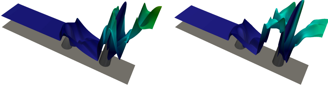
Figure 4.17 – Approximate solution of the 2D dam-break over a double bump experiment, displayed at times t = 0.75\text{s} (left panel) and t = 0.9\text{s} (right panel).
