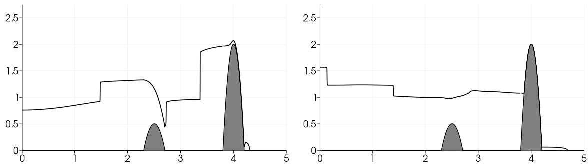
Figure 3.34 – Free surface for the double bump test case at different times. The gray area is the topography. Left panel: solution at t = 0.74s ; right panel: solution at t = 1.70s .
