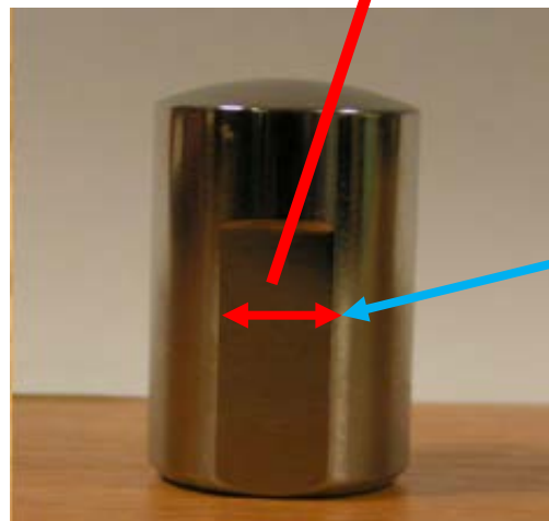
Pin With Relocation Key Way Used To Clock Pin in Jaw Accurately As Possible Between Measurement and Polishing Runs
