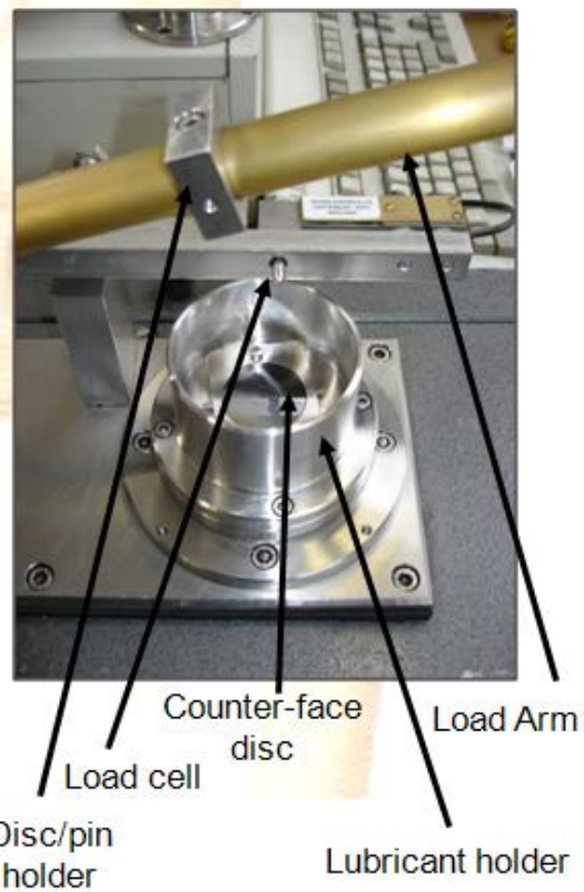
Figure 8.10 Teer Coatings Pin-on-Plate Wear Test Rig
