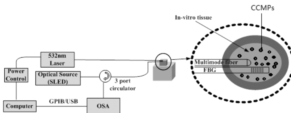
Fig. 1. Schematic of the tissue hyperthermia experiment.
