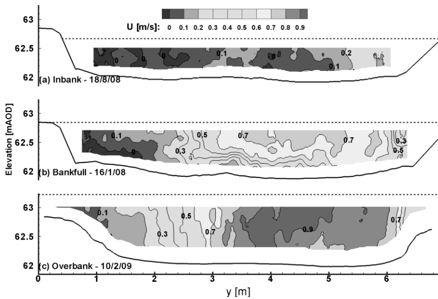
Fig. 7. Contours of the streamwise velocity component ( U ) for the three dates of concern – cross section 2. ( y is the lateral distance from the left hand bank looking downstream).
