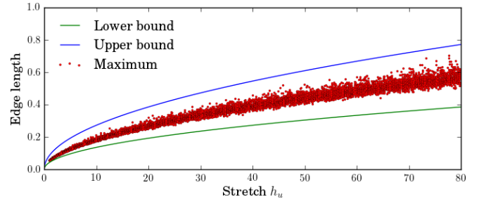
Fig. 6. Edge lengths in a k -nearest foam ( k = 6 ), within a jittered grid of size 32 \times 32 covering the unit square. The metric stretch goes up to an (extreme) value of h_u = 80 . The curves outline the lower and upper bounds.
