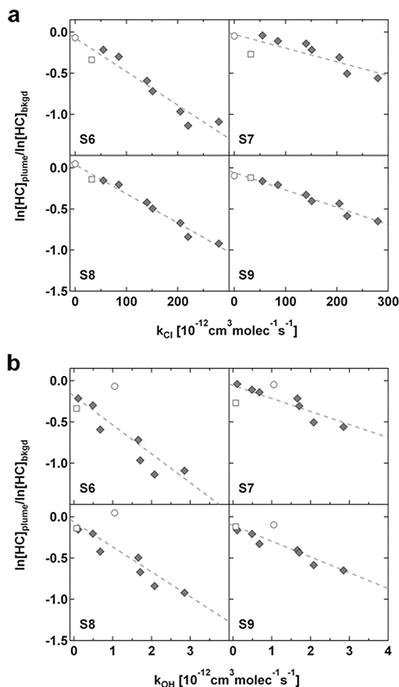
Figure 3. Relationship between NMHC depletions ( \ln([\text{HC}]_{\text{plume}}/[\text{HC}]_{\text{bgd}}) ) and rate of reaction with (a) k_{\text{Cl}} and (b) k_{\text{OH}} for 4 samples (S6–S9) collected within the volcanic plume on 19 May between 11:25 and 11:45 UTC. Open circles denote benzene, open squares denote PCE. Fit parameters are given in Table 2.
