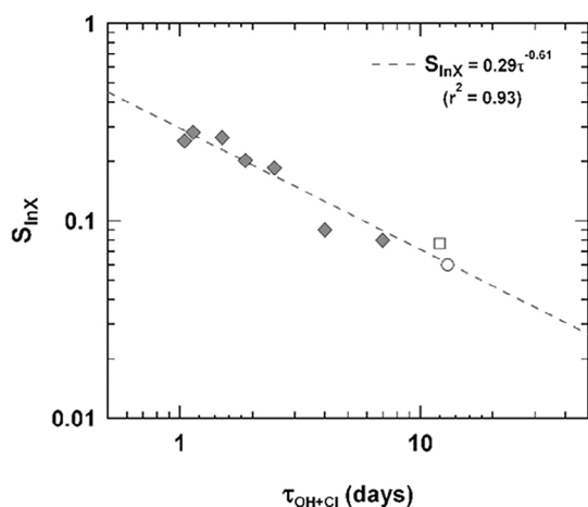
Figure 4. Relationship of plume variability ( S_{\text{InX}} ) and local lifetime ( \tau_{\text{OH} + \text{Cl}} ) for NMHCs measured in samples collected in the volcanic plume during the flight on 19 May, assuming [\text{Cl}] of 2.8 \times 10^4 \text{ Cl cm}^{-3} and an optimized [\text{OH}]/[\text{Cl}] of 37 (see text). Open circles denote benzene, open squares denote PCE.
