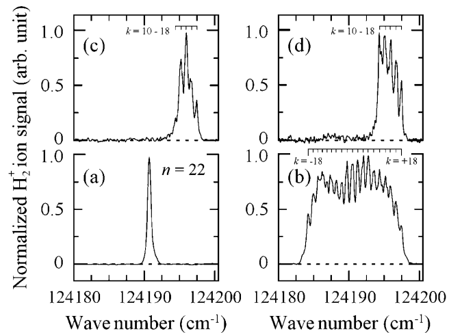
FIG. 3. (a) Field-free n = 22 , \ell = 3 , |M_J| = 3 Rydberg state of \text{H}_2 detected at t_{\text{ion}} = 3 \mu\text{s} . (b) n = 22 , |M_J| = 3 Stark manifold recorded in an electric field of 278 \text{ V/cm} with detection at t_{\text{ion}} = 3 \mu\text{s} . Electrostatically trapped low-field-seeking k = 10\text{--}18 , n = 22 , |M_J| = 3 Stark states of \text{H}_2 detected at t_{\text{ion}} = 50 \mu\text{s} with pulsed potentials of (c) 1.7 and (d) 2.3 \text{ kV} applied for deceleration.
