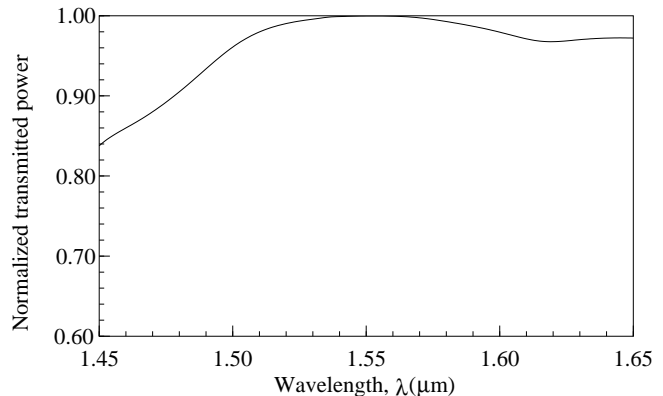
Fig. 5. Wavelength dependence of the normalized transmitted power of the optimized structure in the single-wavelength optimization.
