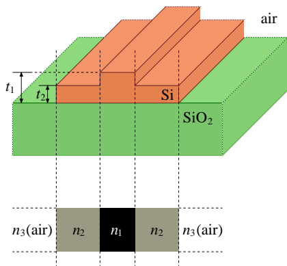
Fig. 2. Optimization model of waveguide crossing.
