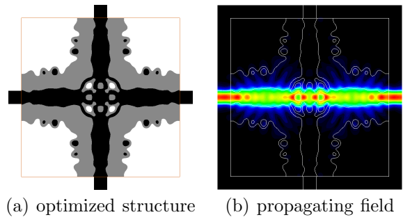
Fig. 4. Optimization results of waveguide crossing at wavelength of 1.55 \mu\text{m} .
