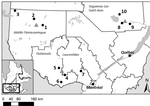
Figure 1. Locations of the study lakes (circles) and sources of climate data (triangles).
