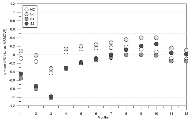
Figure 5. Differences between mean Lake Lacasse \delta^{18}\text{O} in the reference period and mean Lake Lacasse \delta^{18}\text{O} in the future period, for the RCP 4.5 climate scenario and four scenarios of recharge evolution: no change (NC), -33\% in the summer (from June to October; S0), +200\% during the melt period (from January to March) and -4\% in the summer (S1), and +200\% during the melt period and -33\% in the summer (S2).
