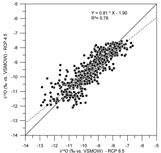
Figure 6. Comparison between monthly results in \delta^{18}\text{O} for both scenarios RCP 4.5 and 8.5 for the 2010–2071 period.
