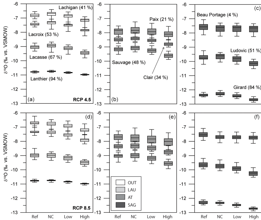
Figure 7. Reference period (Ref; 2010–2040) lake \delta^{18}\text{O} composition and that corresponding to three different future period (2041–2071) recharge scenarios: no change (NC), +14% (Low), and +45% (High), for RCP 4.5 (top) and RCP 8.5 (bottom) scenarios. The values in brackets correspond to the mean G index (percentage of groundwater flow in the total inflow) for each lake calculated for the reference period; left panels show OUT and LAU regions, middle panels AT, and right panels SAG; box whiskers describe median, first, and third quartiles as well as maximum and minimum values.
