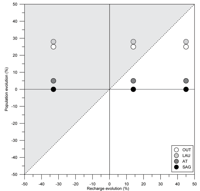
Figure 9. Population growth predictions versus changes in recharge. The shaded area represents the scenarios for which lakes may be under risk of too-high P loading, and therefore at risk of a decrease in water quality. Dots represent lakes in the four study areas for three recharge scenarios.
