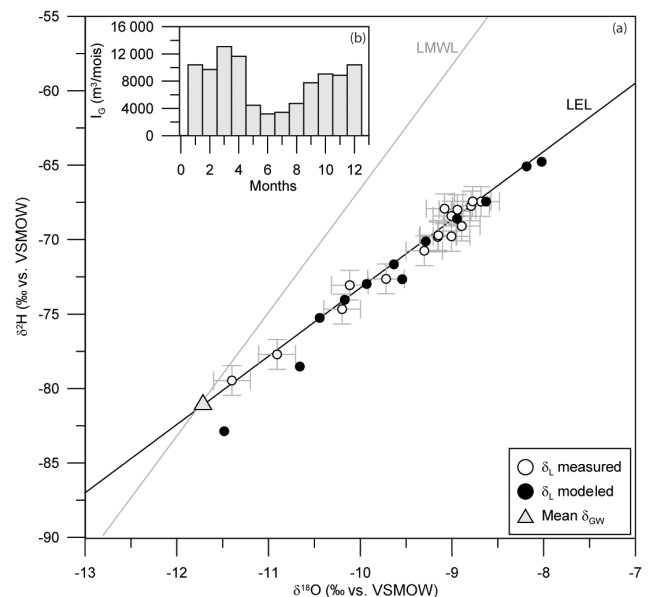
Figure 3. (a) Isotopic composition of Lake Lacasse between June 2015 and May 2016, measured and modeled from stable isotopic mass balance model using climate data from climate model CRCM5 – CanESM2 and scenario RCP 4.5; (b) the pattern of groundwater inflow ( I_G ) to Lake Lacasse (Arnoux et al., 2017b).
