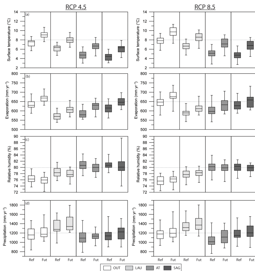
Figure 2. Climate data for the reference (Ref; 2010–2040) and future (Fut; 2041–2071) periods, obtained from CRCM5–CanESM2, with RCP 4.5 (left) and RCP 8.5 (right) scenarios for the four different study areas. The variables are (a) surface air temperature, (b) surface water evaporation (obtained from surface heat flux), (c) surface relative humidity (obtained from surface specific humidity), and (d) precipitation (Martynov et al., 2013; Šeparović et al., 2013); box whiskers describe median, first, and third quartiles as well as maximum and minimum values.
