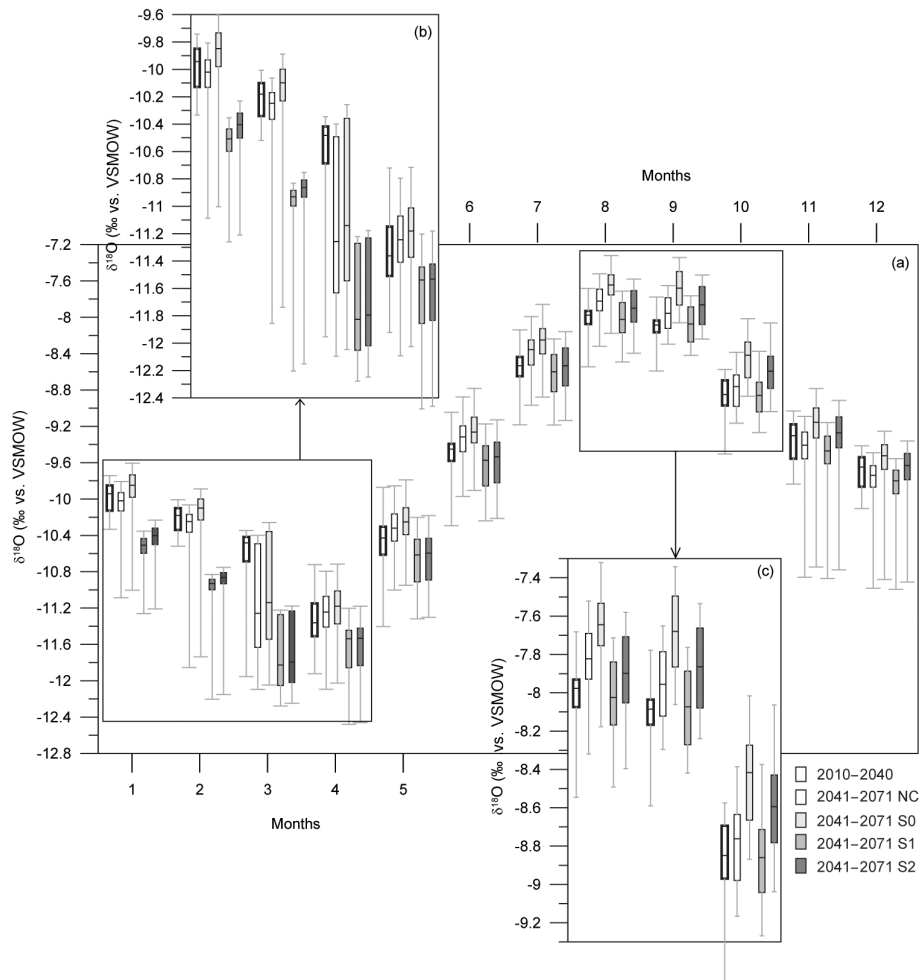
Figure 4. (a) Monthly Lake Lacasse isotopic composition, calculated using RCP 4.5 climatic data, for different periods and various recharge patterns: no change (NC), -33\% in the summer (from June to October; S0), +200\% during the melt period (from January to March) and -4\% in the summer (S1), and +200\% during the melt period and -33\% in the summer (S2); (b) close-up of the winter months; (c) close-up of the summer months; box whiskers describe median, first, and third quartiles as well as maximum and minimum values.
