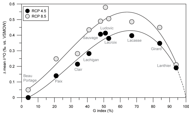
Figure 8. Differences between mean lake \delta^{18}\text{O} in the reference period (2010–2040) and future period (2041–2071), for the higher recharge change scenario, versus lake G indices. RCP 4.5 (black dots) and 8.5 (grey dots) scenarios are represented.
