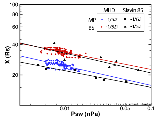
Figure 4. Comparison of BS and MP locations measured by Pioneer 11, Voyager 1 and Voyager 2 [ Slavin et al. , 1985] with those extracted from the MHD model. Lines indicate fits to a power law of the form P_{sw}^\alpha . Values for \alpha are indicated in the figure.
