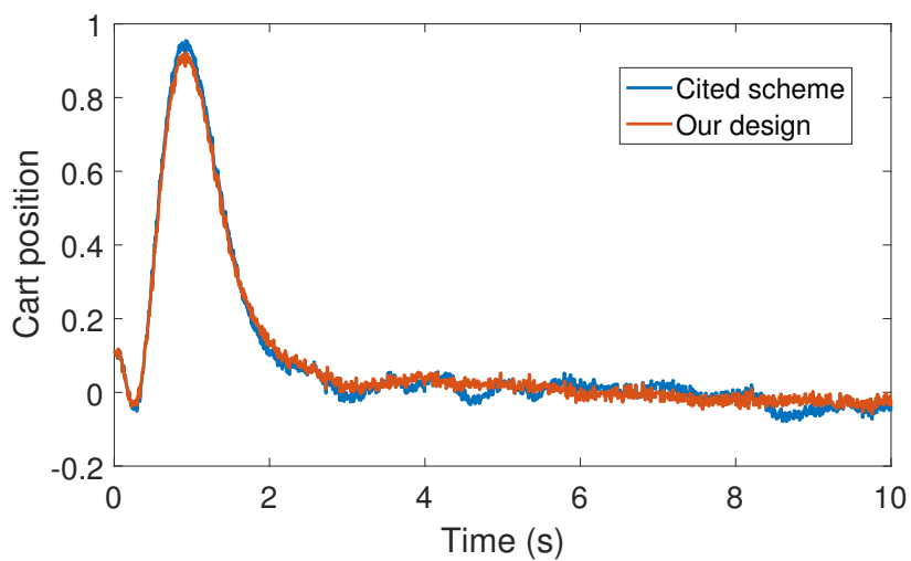
Figure 7. Numerical experiment results (noisy case): cart position (m).
