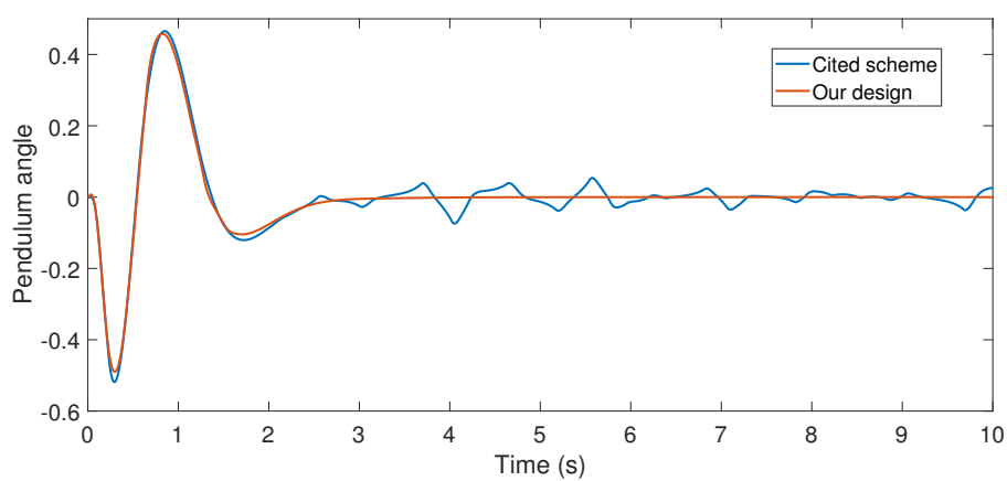
Figure 4. Numerical experiment results: pendulum angle (Rad).
