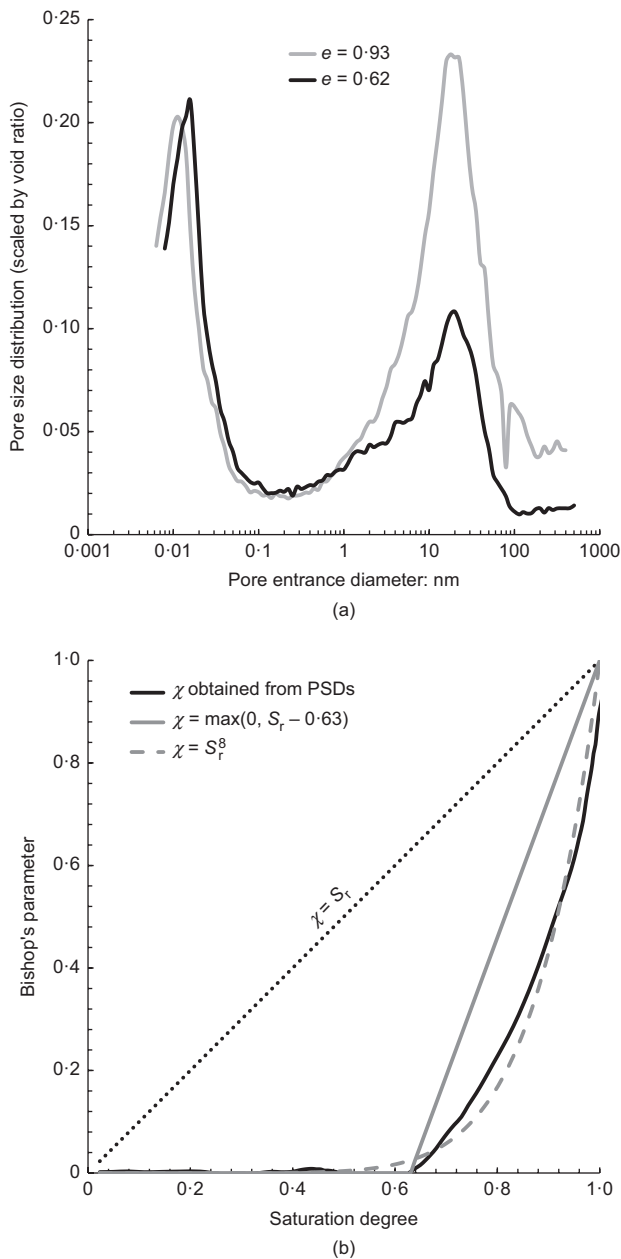
Fig. 6. Determination of Bishop's coefficient for highly active clay (Febex clay): (a) PSD (after Lloret & Villar, 2007); (b) variation of Bishop's coefficient with degree of saturation
