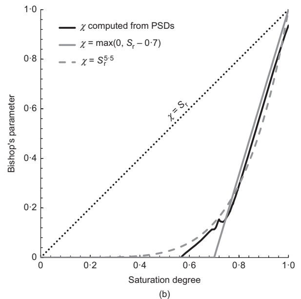
Fig. 5. Determination of Bishop's coefficient for low-plasticity sandy clay (lean clay): (a) PSD (after Li & Zhang, 2009); (b) variation of Bishop's coefficient with degree of saturation
