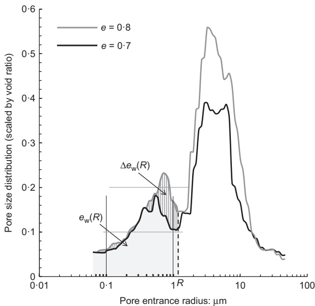
Fig. 3. Pore size distribution of two samples of Jossigny silt compacted at void ratios equal to 0.8 and 0.7 (the PSD has been scaled by the respective value of void ratios)
