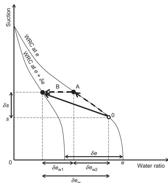
Fig. 1. Partition of total water volume change into components due to suction and deformation only for a path going from the water retention curve (WRC) at e to WRC at e + \delta e
