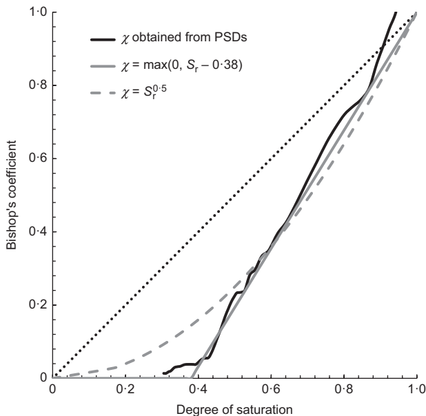
Fig. 4. Variation of \chi with degree of saturation for samples of Jossigny silt compacted at void ratio equal to 0.8
