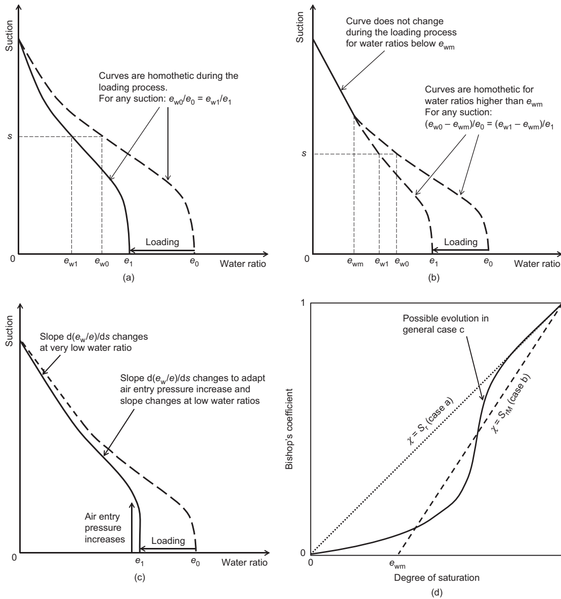
Fig. 2. Schematic variation of Bishop's coefficient for different types of water retention curve strain dependency: (a) water ratio–suction curve that preserves its shape over the whole range of degree of saturation during straining; (b) water ratio–suction curve that preserves its shape over the range of macrostructural degree of saturation and remains constant in the microstructural range; (c) water ratio–suction curve that changes in shape during straining; (d) variation of Bishop's coefficient with degree of saturation for cases a, b and c
