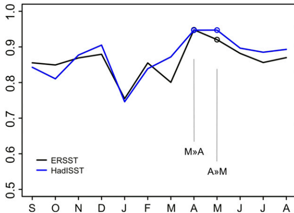
FIG. 9. Lagged correlation of SST anomalies averaged over the TNA ( 5^{\circ} – 15^{\circ} N, 60^{\circ} – 20^{\circ} W; Czaja et al. 2002) between the target month indicated in the x axis and the previous month, computed over the period 1982/83–2010/11, from ERSST.v3b (black) and HadISST.v1.1 (blue). The two highest correlations in the annual cycle are indicated by open circles, which correspond to March > April and April > May.
