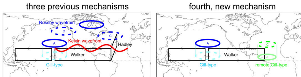
FIG. 1. Schematic diagram of the different mechanisms proposed to explain the ENSO–TNA teleconnection. (left) Previous mechanisms via an extratropical Rossby wave train (rotational circulation; blue); through an atmospheric bridge involving changes in the Pacific Walker and Atlantic Hadley cells (divergent circulation; black); and via the tropospheric temperature mechanism, which is mediated by the propagation of a Kelvin wave front (equatorial dynamics; red). (right) New mechanism via the remote Gill-type response to the ENSO zonally compensated heat source over the Amazon basin, associated with changes in the Pacific Walker cell (tropical dynamics; green). Note that in the Gill-type responses, over both the tropical Pacific and Atlantic, only the anomalous circulations in the Northern Hemisphere are drawn. Thin arrows indicate the direction of the divergent cells. Solid (dashed) circles represent anticyclonic A (cyclonic C) circulations associated with high (low) pressure systems.
