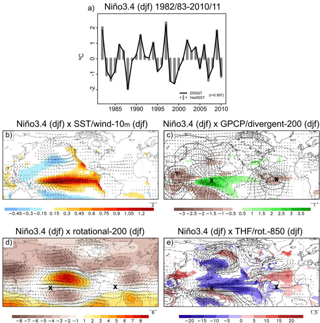
FIG. 2. (a) Niño-3.4 SST index in DJF from ERSST.v3b (black lines) and HadISST.v1.1 (gray bars). Regression maps of (b) SST ( ^{\circ}\text{C} ; shading) and surface wind at 10 m ( \text{m s}^{-1} ; vectors); (c) precipitation ( \text{mm day}^{-1} ; shading), velocity potential [ \text{m}^2 \text{s}^{-1} ]; contours with contour interval ( \text{ci} ) = 0.3 \times 10^6 \text{ m}^2 \text{ s}^{-1} ], and divergent wind ( \text{m s}^{-1} ; vectors) at 200 hPa; (d) streamfunction ( \text{m}^2 \text{ s}^{-1} ; contours with \text{ci} = 1 \times 10^6 \text{ m}^2 \text{ s}^{-1} ) and rotational wind ( \text{m s}^{-1} ; vectors) at 200 hPa; and (e) THF ( \text{W m}^{-2} ; shading; latent plus sensible where downward is positive), streamfunction ( \text{m}^2 \text{ s}^{-1} ; contours with \text{ci} = 0.3 \times 10^6 \text{ m}^2 \text{ s}^{-1} ), and rotational wind ( \text{m s}^{-1} ; vectors) at 850 hPa anomalies in DJF onto the DJF Niño-3.4 index. Statistically significant areas at 95% confidence level are gridded for shading and vectors in (b), (c), and (e) and bolded/shaded for contours in (c)–(e). Thick, black crosses in (c)–(e) stand for the region of max divergence/convergence in the tropical Pacific/Amazon basin.
