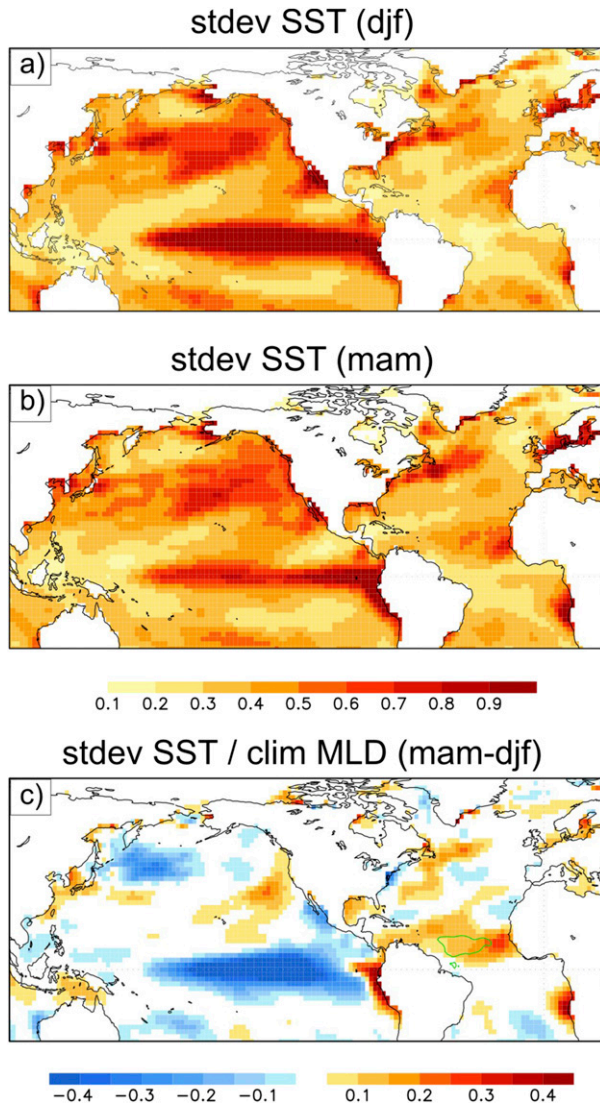
FIG. 6. Std dev of SST ( ^{\circ}\text{C} ; shading) in (a) DJF and (b) MAM, and (c) its difference, over the period 1982/83–2010/11. Areas in the TNA region where the MLD is deeper in MAM as compared to DJF are contoured in (c).
