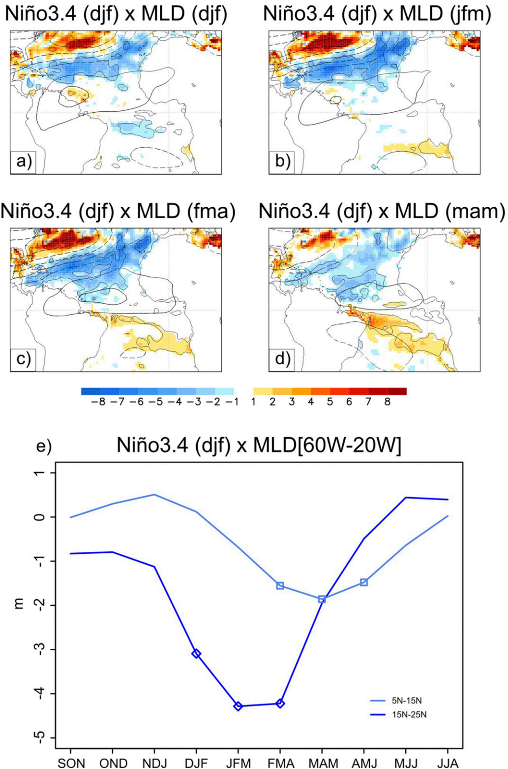
FIG. 5. Regression map of MLD (m; shading) anomalies in (a) DJF, (b) JFM, (c) FMA, and (d) MAM onto the DJF Niño-3.4 index. Statistically significant areas at 95% confidence level are contoured. In each panel the regression of streamfunction anomalies at 850 hPa ( \text{m}^2 \text{s}^{-1} ; contours with \text{ci} = 0.3 \times 10^6 \text{m}^2 \text{s}^{-1} ) is plotted, as in Figs. 2e and 4 (right). (e) Regression of MLD anomalies zonally averaged over the TNA domain 60°–20°W (Czaja et al. 2002) in the 5°–15°N (light blue) and 15°–25°N (dark blue) latitudinal bands. Symbols indicate statistically significant anomalies at 95% confidence level.
