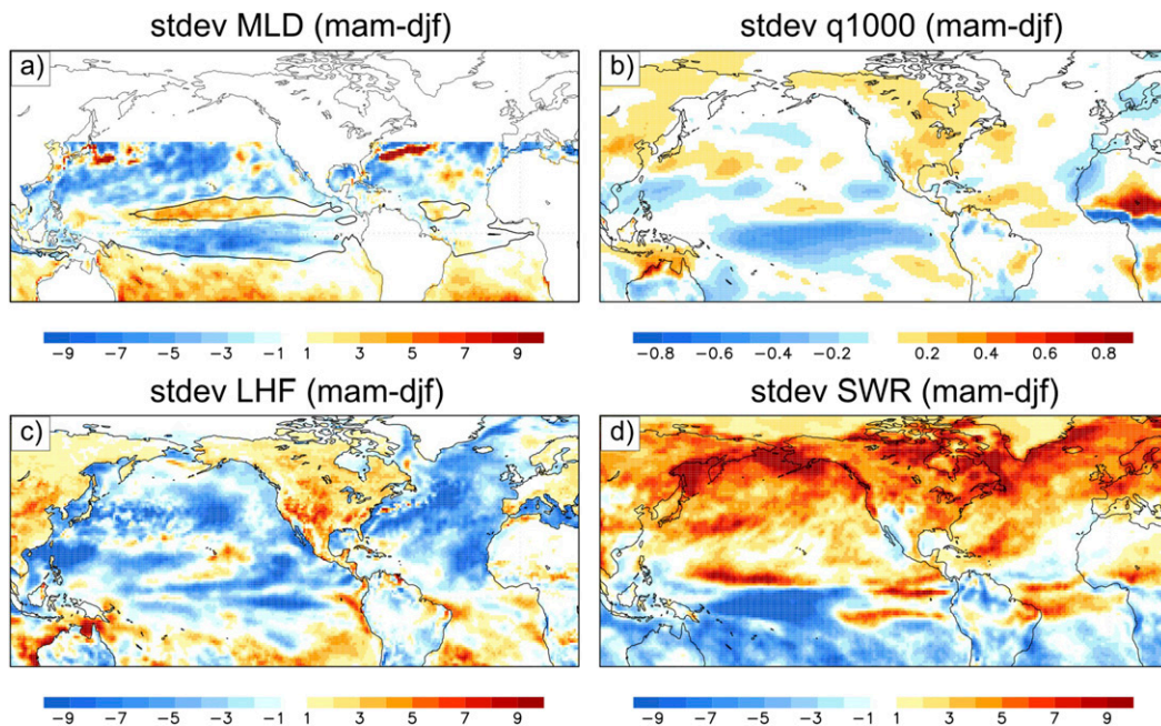
FIG. 8. As Fig. 6c, but for (a) MLD (m), (b) specific humidity at 1000 hPa q_{1000} ( \text{g kg}^{-1} ), (c) surface LHF ( \text{W m}^{-2} ), and (d) SWR ( \text{W m}^{-2} ). Regions where MLD is deeper in MAM as compared to DJF are contoured in (a).
