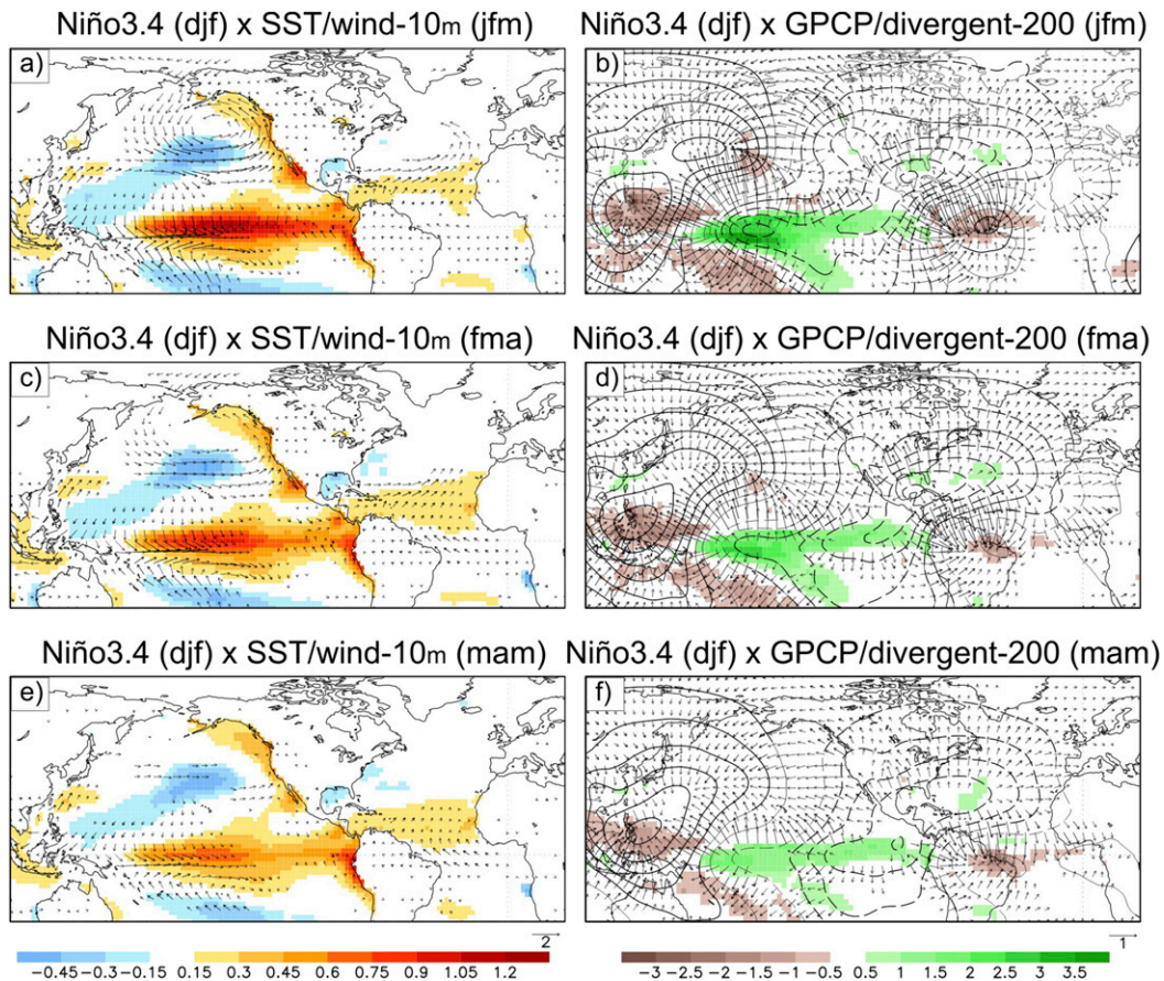
FIG. 3. Regression maps of (left) SST ( ^{\circ}\text{C} ; shading) and surface wind at 10 m ( \text{m s}^{-1} ; vectors) and (right) precipitation ( \text{mm day}^{-1} ; shading), velocity potential ( \text{m}^2 \text{s}^{-1} ; contours with \text{ci} = 0.3 \times 10^6 \text{ m}^2 \text{ s}^{-1} ), and divergent wind ( \text{m s}^{-1} ; vectors) at 200 hPa anomalies in (top) JFM, (middle) FMA, and (bottom) MAM onto the DJF Niño-3.4 index. Statistically significant areas at 95% confidence level are gridded for shading and vectors, and bolded for contours.
