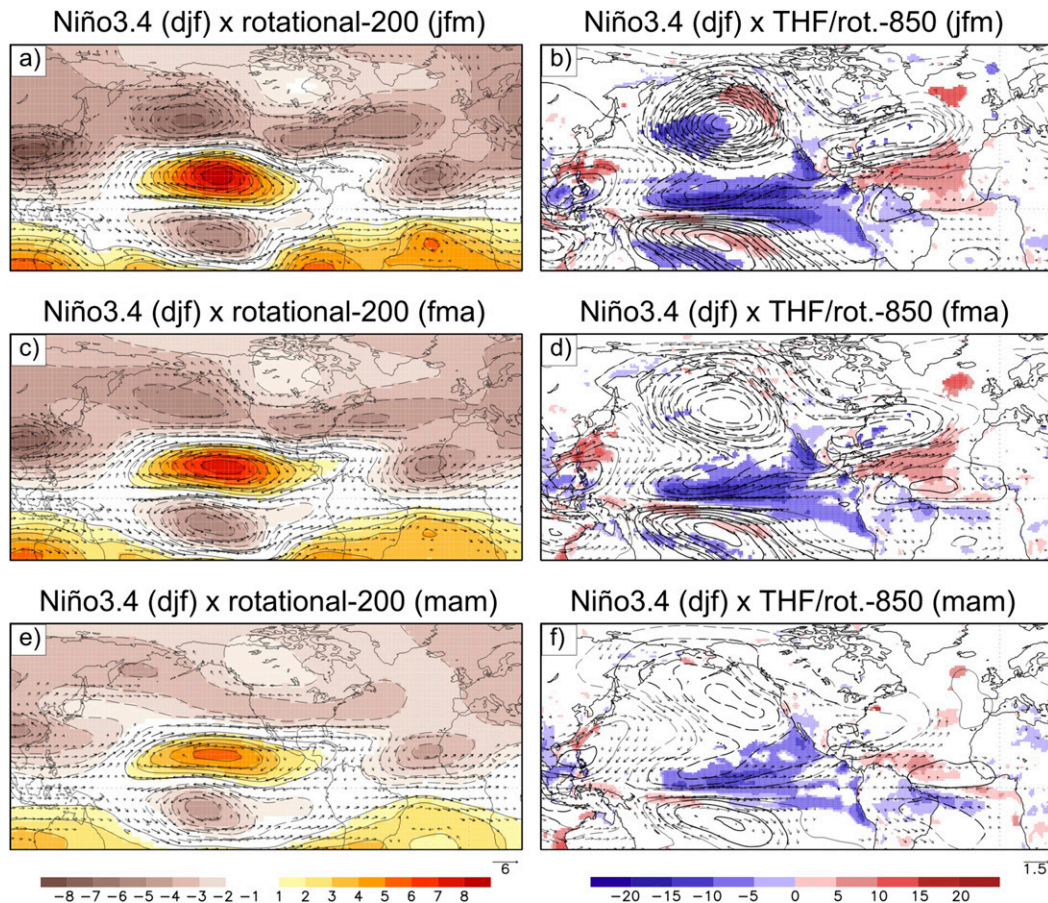
FIG. 4. Regression maps of (left) streamfunction ( \text{m}^2 \text{s}^{-1} ; contours with \text{ci} = 1 \times 10^6 \text{ m}^2 \text{ s}^{-1} ) and rotational wind ( \text{m s}^{-1} ; vectors) at 200 hPa anomalies and (right) THF ( \text{W m}^{-2} ; shading; latent plus sensible where downward is positive), streamfunction ( \text{m}^2 \text{ s}^{-1} ; contours with \text{ci} = 0.3 \times 10^6 \text{ m}^2 \text{ s}^{-1} ), and rotational wind ( \text{m s}^{-1} ; vectors) at 850 hPa anomalies in (top) JFM, (middle) FMA, and (bottom) MAM onto the DJF Niño-3.4 index. Statistically significant areas at 95% confidence level are gridded for shading and vectors, and shaded/bolded for contours [(left) and (right), respectively].
