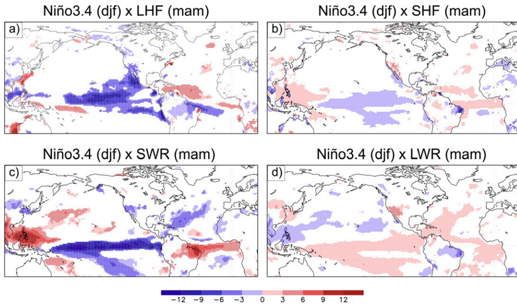
FIG. 7. Regression map of surface (a) latent heat flux (LHF), (b) sensible heat flux (SHF), (c) shortwave radiation (SWR), and (d) longwave radiation (LWR) anomalies in MAM onto the DJF Niño-3.4 index; downward is positive ( \text{W m}^{-2} ). Statistically significant areas at 95% confidence level are gridded.
