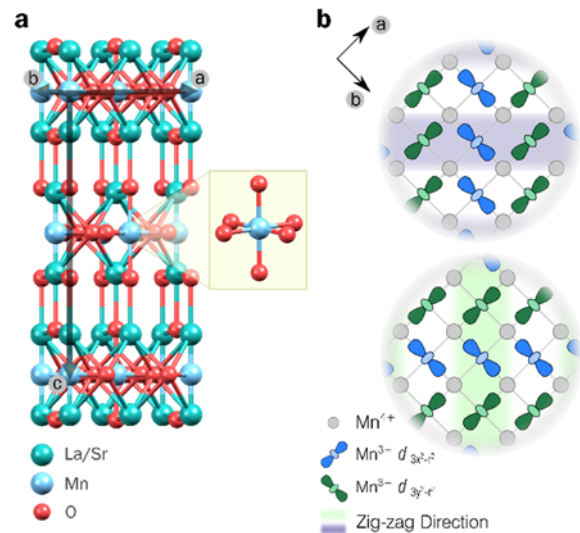
Figure 1: The crystal structure of LSMO (a). The \text{Mn}^{3/4+} ion has octahedral coordination with oxygen (top inset), while the in-plane Mn-O bonds are slightly distorted from 90^\circ (bottom inset). (b) Two of the four possible domains below T_{\text{CO/OO}} . The two other domains are related through a translation of the charge ordered state by one Mn lattice site.
