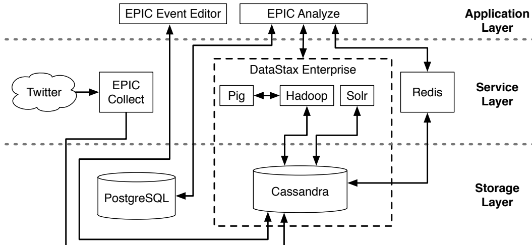
FIGURE 2.1: Project EPIC Software Infrastructure
