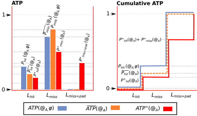
Fig. 2. Relation among ATP(\@_A, \phi) , ATP^+(\@_A) and \overline{ATP}(\@_A) .
