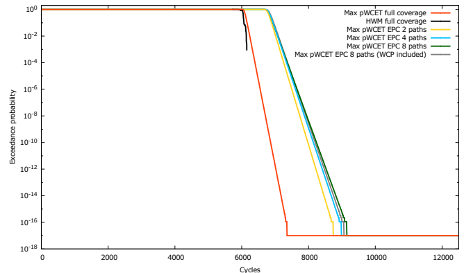
Fig. 5. EVT projections: full-path vs EPC over-approximations.
