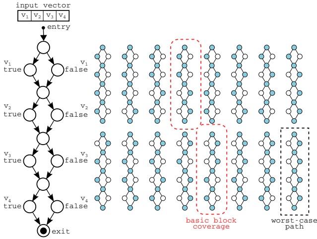
Fig. 4. Overview of MultiBranch structure.
