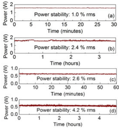
Fig. 8. Passive power stability of the idler at room temperature for (a) 30 min, and (b) >3 h, and at 200 °C for (c) 60 min, and (d) >4 h.
