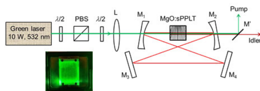
Fig. 1. Schematic of the rapidly tunable cw near-IR OPO. \lambda/2 : half-wave plates; PBS, polarizing beam-splitter; L, lens; M_{1-4} , mirrors; M' : dichroic mirror. Inset: Laboratory picture of the mounted MgO:sPPLT crystal.
