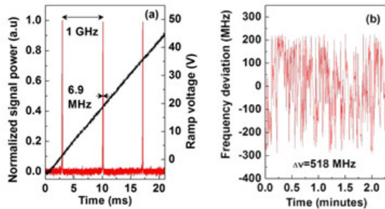
Fig. 9. (a) Single-frequency spectrum, and (b) Frequency stability of the signal at 837 nm.
