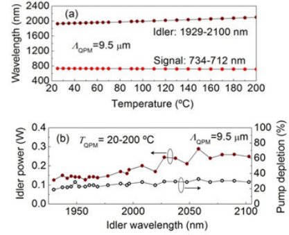
Fig. 6. (a) Temperature tuning, and (b) Variation of idler power and pump depletion across the tuning range for the longest grating period of \Lambda=9.5 \mu\text{m} .
