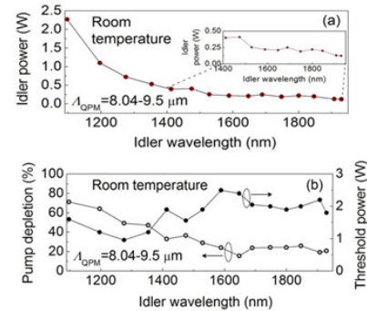
Fig. 3. Variation of (a) Idler power, and (b) Pump depletion and threshold power across the grating tuning range at room temperature.
