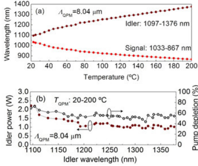
Fig. 4. (a) Temperature tuning, and (b) Variation of idler power and corresponding pump depletion across the tuning range for the shortest grating period of \Lambda=8.04 \mu\text{m} .
