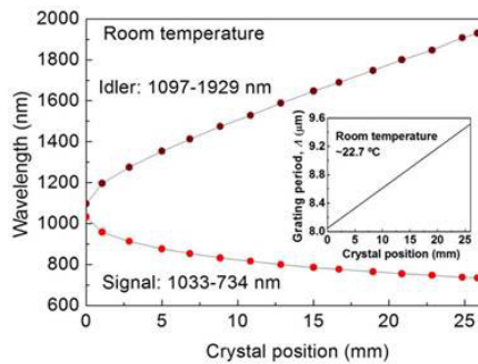
Fig. 2. Rapid wavelength tuning with crystal translation at room temperature. Inset: Theoretically calculated grating period corresponding to the crystal position used.
