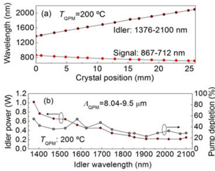
Fig. 5. (a) Grating tuning, and (b) Idler power and pump depletion across the tuning range at a fixed crystal temperature of 200 ^{\circ}\text{C} .
