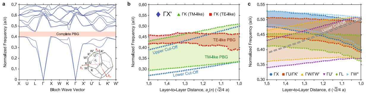
Figure 2. Bandstructure analysis of the woodpile PhC structure. (a) Numerically calculated band structure of the woodpile PhC with \text{Al}_2\text{O}_3 rods. The lower right inset depicts the first Brillouin zone of the woodpile structure. (b) The dependency of the layer-to-layer distance onto the longitudinal and transverse cut-off frequencies. The TM-like and TE-like PBGs in the transverse directions are highlighted with light green and red colored areas. (c) The PBG variations for other directions. The dashed white line indicates the upper cut-off frequencies in the \Gamma - X' direction.
