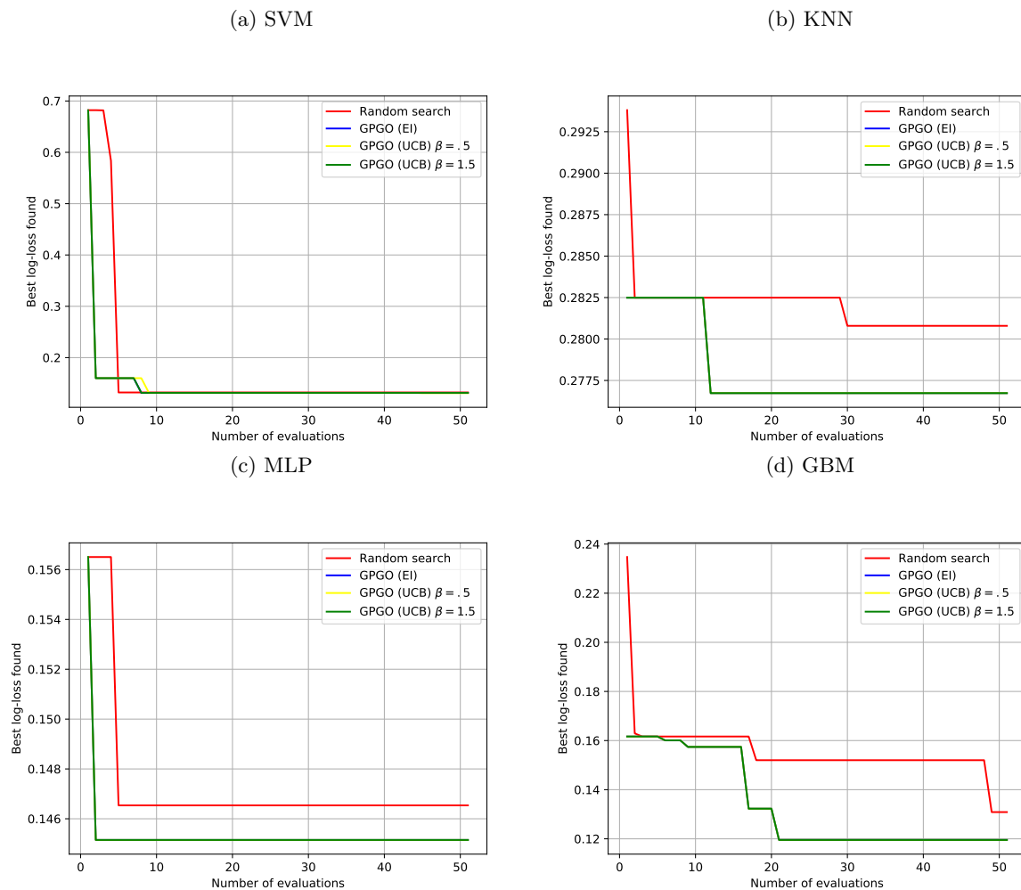
Figure 4.11: Benchmarking results for the breast cancer dataset.
