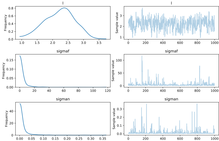
Figure 5.4: Posterior sampled distributions of hyperparameters using MCMC.
