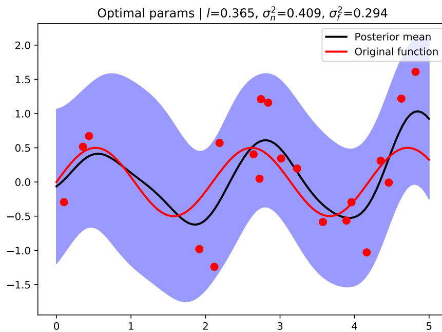
Figure 5.3: Gaussian Process regression of noisy inputs with pyGPGO.
