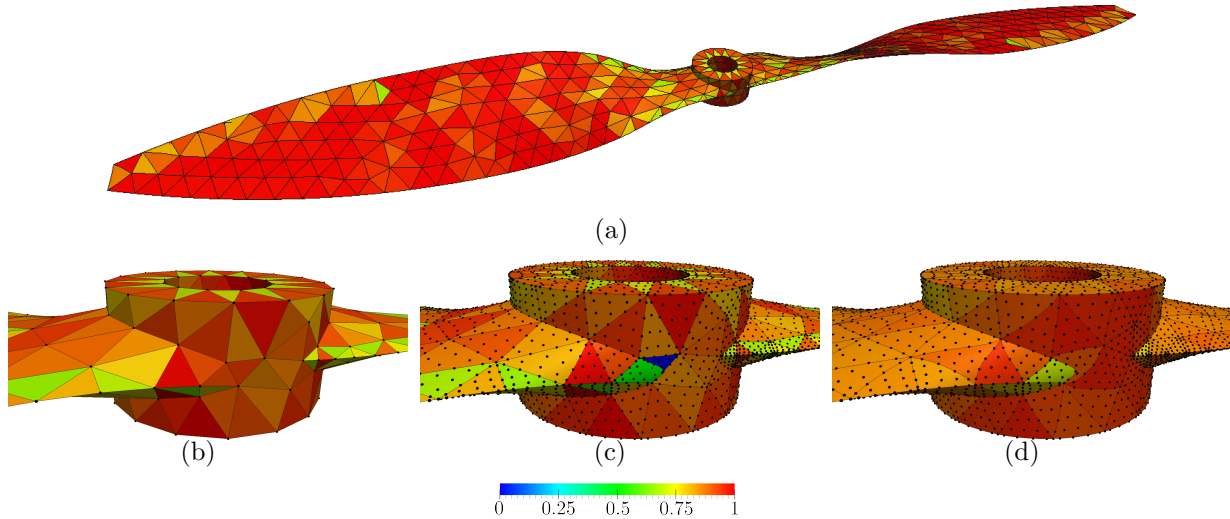
Figure 4. Process for the generation of an order 5 surface mesh on a propeller. The elements are colored according to the shape quality measure. (a) Overview of the optimized high-order mesh. Detail of the (b) initial linear mesh, (c) initial high-order mesh, and (d) optimized high-order mesh.
