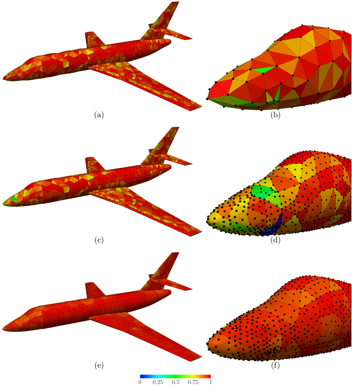
Figure 3. Process for the generation of an order 3 surface mesh on a Falcon aircraft. The elements are colored according to the shape quality measure. (a,b) Initial linear mesh. (c,d) Initial order 3 mesh obtained after increase the order of the initial linear mesh. (e,f) Optimized order 3 mesh.
