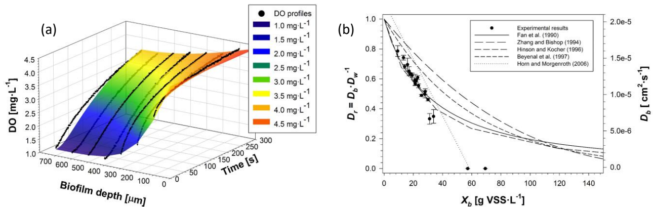
Figure 2. a) Simulated (mesh) and experimental (dots) oxygenation profiles for the calculation of the oxygen diffusivity in a biofilm section. b) Effect of biofilm density (measured as volatile suspended solids (VSS) per liter) on the biofilm diffusivity, experimental data vs empirical correlations. Diffusion coefficient is also presented as a relative diffusivity ( D_r ), normalized using oxygen diffusivity in water ( D_w ).
