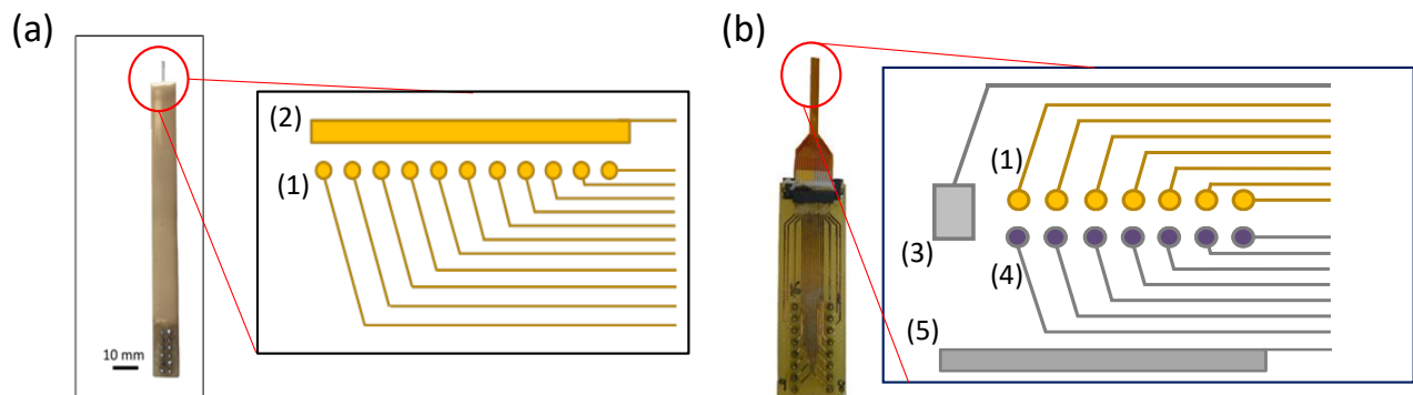
Figure 1. Schematic of the MEA sensors prototypes used in this study. a) DO MEA; b) DO-pH MEA. (1) Gold-disk electrodes, (2) internal gold counter electrode, (3) internal platinum pseudo-reference electrode, (4) iridium oxide coated electrodes and (5) internal platinum counter electrode.
