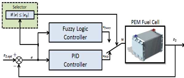
Figure 6. Structure of the hybrid Fuzzy-PID controller
