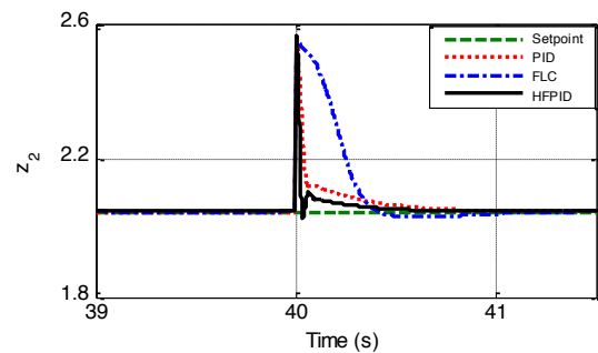
Figure 10. The magnified plot of oxygen excess ratio variation at t=40 s
