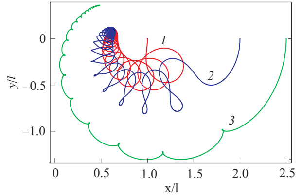
Fig. 2. Three-body dynamics from the solution of Eq. (9), for a system with L/\ell = 20 , \alpha = 0.01 , b = 0.02 , \omega = 1 , and \Omega_G = 0.0287 . The original vortex (1) was positioned at (1,0)\ell , the antivortex (2) at (2,0)\ell , and the newborn vortex (3) at (2.5,0)\ell .
