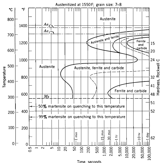
Figure 12. Isothermal Transformation Diagram for 0.30C – 2Cr Steel (U.S. Steel Corporation).
