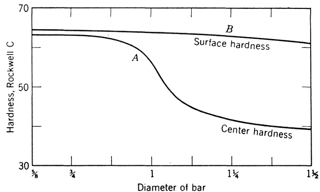
Figure 11. Center vs. Surface Hardness of Carbon-Moly Steel Oil Quenched (After Grossman).
