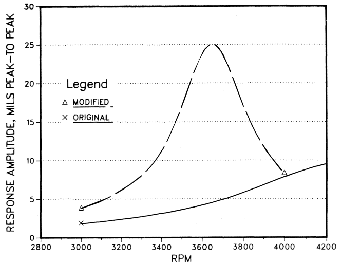
Figure 11. Predicted Unbalance Response of Generator Shaft.
