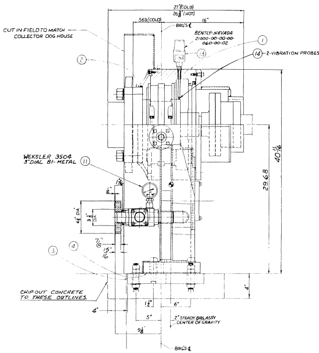
Figure 19. Final Outline—Side View.
