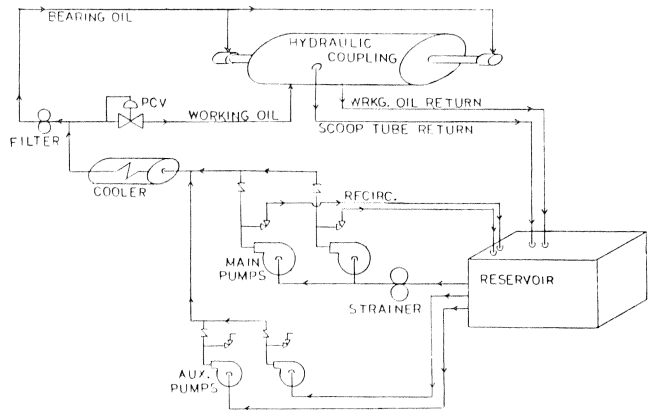
Figure 4. Hydraulic Coupling Oil Circuit Flow Diagram.
