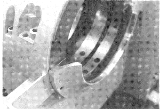
Figure 18. Bearing Housing and Seals.
